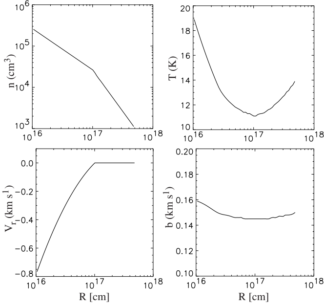
Fig. 2. Physical structure of the test model 2. Upper left: density, lower left: velocity, upper right: temperature, lower right: turbulent line width b [km s ^{-1} ]. Changes in the density and velocity distributions are seen at the point where infall starts. The temperature of the gas at the inside rises due to the infall while the outside is heated by the interstellar radiation.
