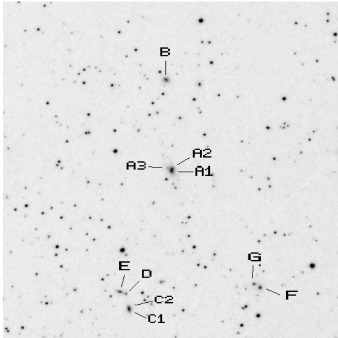
Fig. 2. The field around B2 1637+29, reproduced from the Digital Sky Survey. The image size is 15 by 15 arcminutes. A letter identifies the galaxies listed in Table 1.
