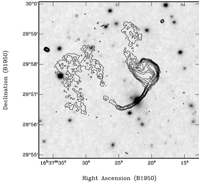
Fig. 1. The radio source B2 1637+29, superposed on an optical image reproduced from the Digital Sky Survey.
