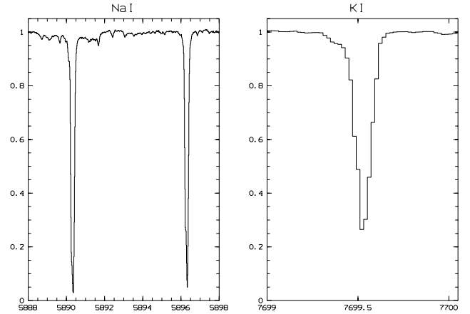
Fig. 1. Normalized UVES spectra of the Na I (D1 and D2) and KI (7698.98 Å) interstellar lines toward HD 147889. The Na I line is saturated (from the D1 and D2 line ratio) but the KI line is not. Both lines show only one narrow velocity component, indicative of a single cloud structure in this line of sight.
