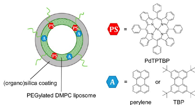
Figure 1. Schematic representation of (organo)silica-coated liposomes containing photosensitizer (PS; PdTPTBP) and annihilator chromophores (A; perylene or TBP). PdTPTBP = palladium tetraphenyltetrazaborporphyrin, TBP = 3,5,8,11-tetra( tert -butyl)perylene.
