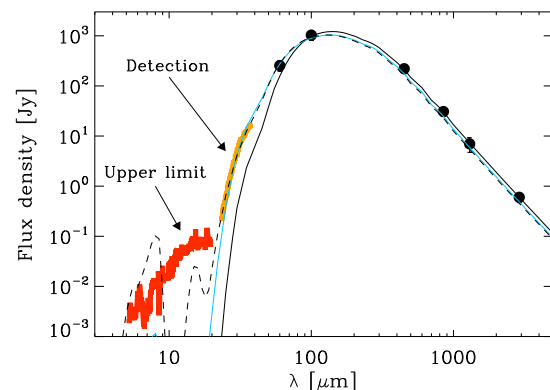
Figure 2: Spitzer/IRS observations of IRAS 16293–2422 and models for its SED. The black solid line is the best fit model by Schöier et al. (2002), the grey solid line is the Schöier et al. model with a 600\text{ AU} (radius) cavity, and the dashed line is the cavity model with a central 500\text{ K} black body.
