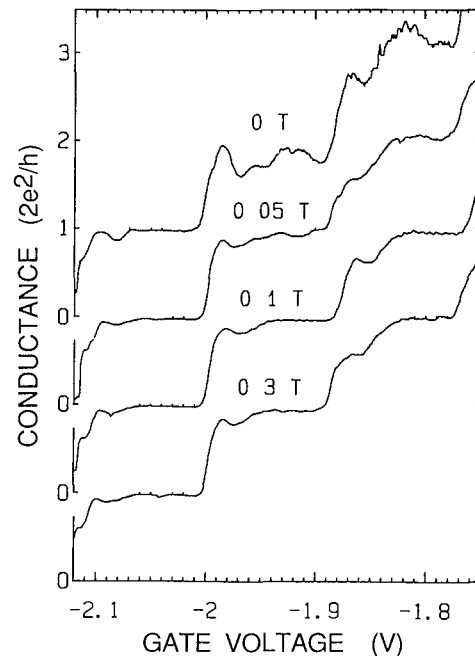
FIG. 9. Improvement of the conductance quantization by the application of a magnetic field, measured at 40 mK.
