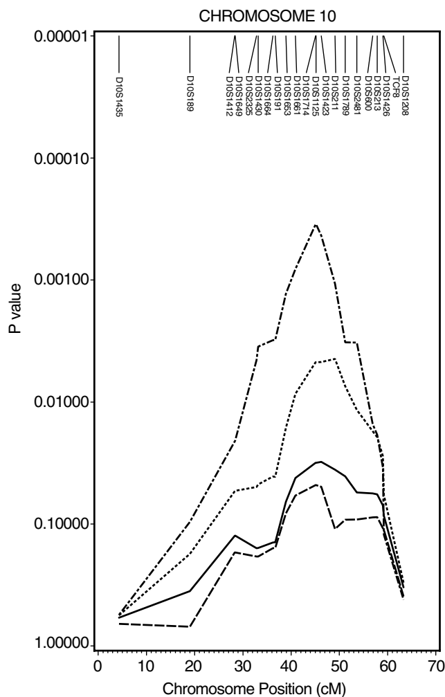
Fig. 4. Fine-mapping of chromosome 10. Shown are P -values for statistics A (irregular), B (long dashed), C (short dashed), and D (solid) by centimorgan (cM) across the region identified in the genome scan.
