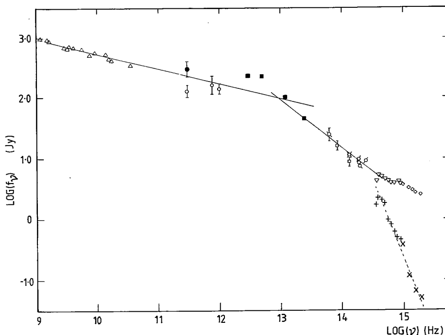
FIG. 1.—Radio, infrared, optical, and ultraviolet spectrum of the Crab nebula. Data are from the following sources: \Delta , Baars and Hartsuijker (1972); \bullet , Werner et al. (1977); \circ , Wright et al. (1979); \blacksquare , IRAS ; open circle with \diagdown , Grasdalen (1979); \square , Ney and Stein (1968); open circle with \diagup , Becklin and Kleinmann (1968); \nabla , Scargle (1969), corrected for extinction; + , Scargle (1969), uncorrected for extinction; \diamond , Wu (1981), corrected for extinction; \times , Wu (1981), uncorrected for extinction.
