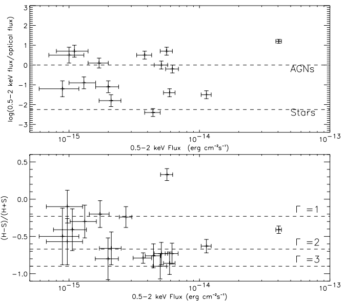
Fig. 2. Upper panel: the soft X-ray to optical flux ratio versus the soft X-ray flux. The dotted lines give the typical ratios for AGN (upper) and stars (lower) as determined by Stocke et al. (1991). Lower panel: the hardness ratio (H - S)/(H + S) versus the soft band flux for all sources. The dashed lines show power law models with different photon indices ( \Gamma ) computed assuming the galactic value N_H = 4.5 \times 10^{20} cm -2 .
