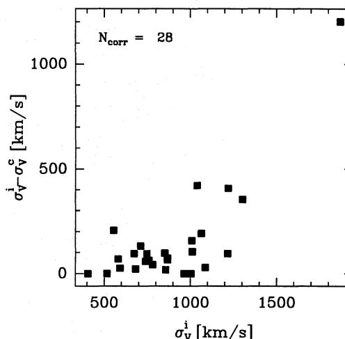
Fig. 4. The decrease in velocity dispersion as a result of the removal of interlopers, versus the initial, uncorrected value of the velocity dispersion.
