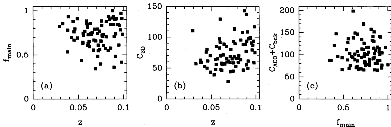
Fig. 2. a The dependence of f_{\text{main}} (the fraction of galaxies in the largest system) on the redshift of the main system. b The dependence of intrinsic richness count C_{3D} on the redshift of the system. c The dependence of C_{\text{ACO}} + C_{\text{bck}} on f_{\text{main}} .
