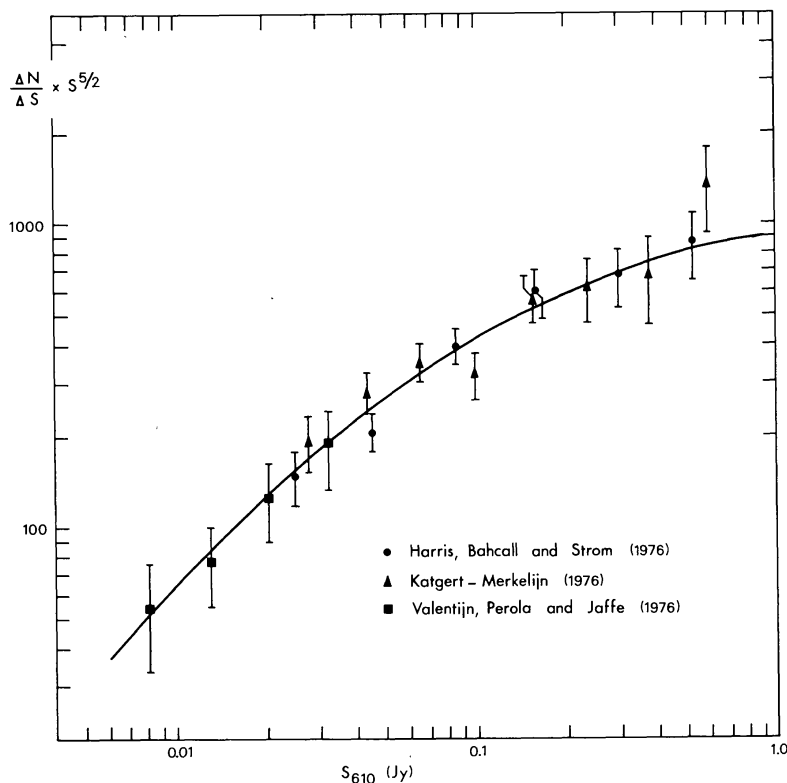
Fig. 1. WSRT 610 MHz differential counts. The solid line describes eq.(1).
