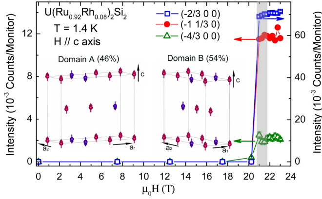
FIG. 3. Field dependence of the intensity of representative magnetic reflections observed in \text{U}(\text{Ru}_{0.92}\text{Rh}_{0.08})_2\text{Si}_2 single crystal at 1.4 K with the field applied along the c axis. In the inset we show the field-induced magnetic structure consisting of two single- \mathbf{Q} domains. The shaded area denotes the range of fields where the MT occurs with lowering the field.
