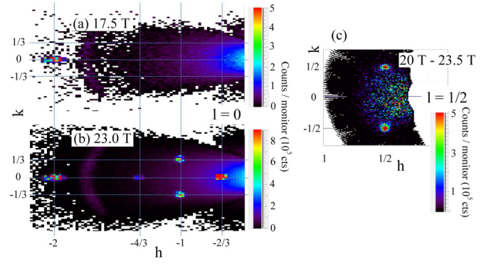
FIG. 2. (a) Portion of the l=0 reciprocal space plane of \text{U}(\text{Ru}_{1-x}\text{Rh}_x)_2\text{Si}_2 covered by the first geometry with field along the c axis in the forward direction, showing the color-coded intensity of diffracted neutrons at 17.5 T, and (b) at 23 T, both at 1.4 K. (c) The intensity difference for the l=1/2 reciprocal space plane recorded with fields of 20 and 23.5 T in the second geometry with the field inclined from the c axis.
