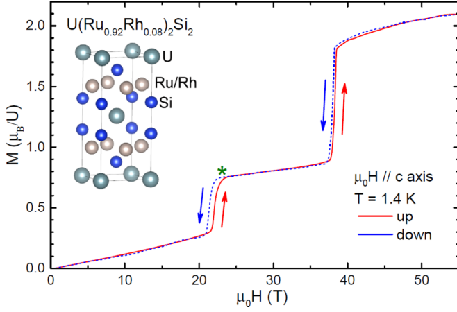
FIG. 1. The field dependence of the magnetization of \text{U}(\text{Ru}_{0.92}\text{Rh}_{0.08})_2\text{Si}_2 measured with field applied along the c axis at 1.4 K. The star marks the field at which the neutron experiment has been performed. In the inset the tetragonal crystal structure adopted by the system is shown.
