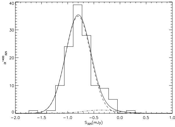
Fig. 9. Spectral index distribution ( S > 0.05 Jy) comparison with De Breuck et al. (2000) Gaussian fits, based on the WENSS/NVSS surveys. Dashed line and dashed-dotted line show the spectral index distribution of the steep-spectrum and the flat-spectrum radio source population respectively (De Breuck et al. 2000).
