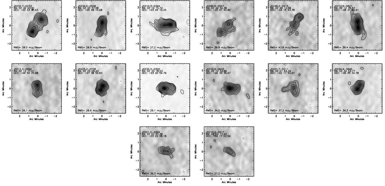
Fig. A.2. The multiple component sources in the 74 MHz source list larger than 60'', sorted in decreasing angular size order. Contours corresponds to levels of 3\sigma \times (-1.4, -1, 1, 1.4, 2, 2.8, 4, 5.6, 8, 11, \dots) and greyscale is scaled from -3\sigma to the maximum value in the image. On the top-left corner of each images appears the name of the corresponding source in the source list, as well as its mean coordinate. The local noise level is shown on the bottom of each image.
