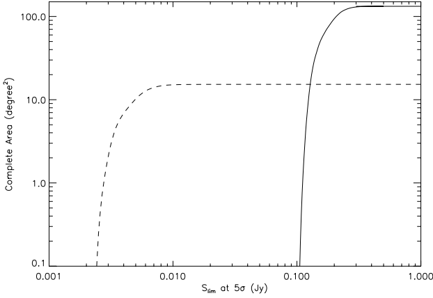
Fig. 2. Area as a function of limiting flux density per beam at 5\sigma . The full line corresponds to the 74 MHz survey whereas the dashed one corresponds to the 325 MHz survey.
