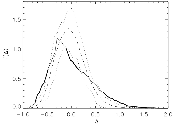
Fig. 3. Plotted here are the (normalised) projected density distribution function (PDDF) of the whole sample of 874 LBGs (solid line) and the combined PDDF of 20 equally sized mock samples (dashed line is mean, dotted lines are mean \pm 3\sigma , where \sigma is the standard deviation between the mock samples). At several intervals, the PDDF of the LBG sample deviates from the mock samples by more than 3\sigma (thick solid line). The smoothed LBG distribution has relatively less area with a density close to mean, relatively more area out to higher densities and relatively more area with lower densities, which characterizes the presence of compact overdensities with high peaks and extended underdensities.
