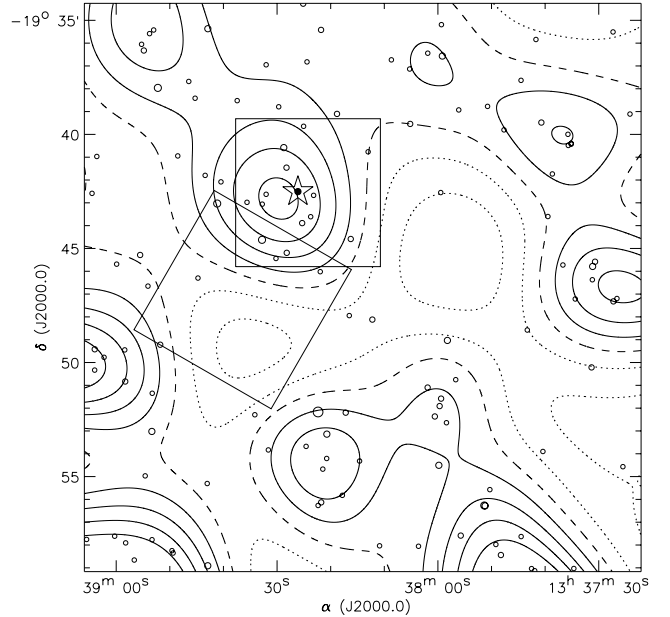
Fig. 1. Projected distribution of 125 bright LBGs (open circles; diameter scales with brightness; 21.5 < i' < 25.0 ) in the TN J1338–1942 field, including TN J1338–1942 (filled circle within star). The projected density contours (curved lines), obtained by Gaussian smoothing, reveal overdense (solid lines; \Delta = 0.25, 0.50, 0.75, 1.00 from edge to center) and underdense regions (dotted lines; \Delta = -0.25, -0.50, -0.75 from edge to center) relative to a mean density of 0.21 per square arcminute (dashed line). TN J1338–1942 inhabits a significant overdense area, probably associated with the protocluster found by Venemans et al. (2002). The rectangles represent the two fields that were used by Venemans et al. (2002) and Venemans (2005) to search for LAEs.
