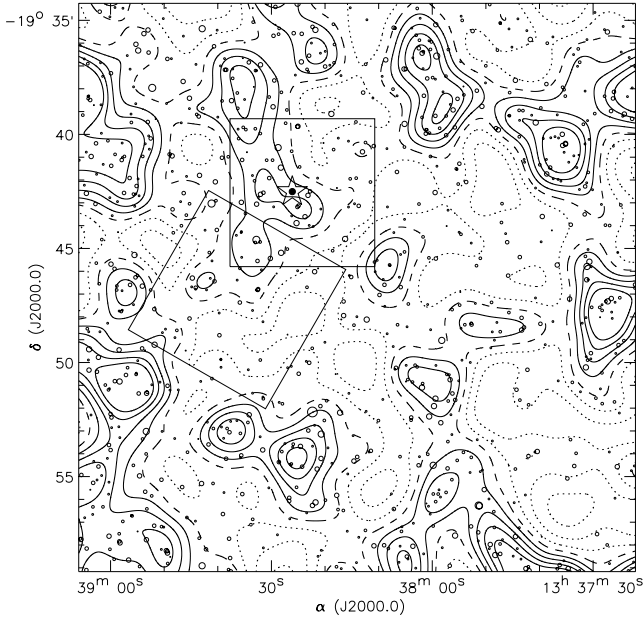
Fig. 2. Projected distribution of 874 LBGs with 21.5 < i' < 26.5 in the TN J1338–1942 field, similar to Fig. 1. The contours are relative to a mean density of 1.47 per square arcminute (dashed line). Like in Fig. 1, TN J1338–1942 inhabits a significant overdense area, probably associated with the protocluster found by Venemans et al. (2002).
