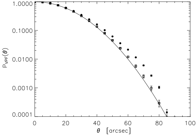
Fig. 4. The two-dimensional void probability function (VPF) of the LBG sample (filled dots; error bar is Poissonian error), compared with the mean VPF of 20 mock samples (open squares; error bar is combination of Poissonian error and standard deviation between mock catalogs) and the theoretical VPF for Poissonian distributions (solid line). For radii \theta > 40'' , the underdensities in the projected LBG distribution are significantly larger than the underdensities in mock and Poissonian distributions.
