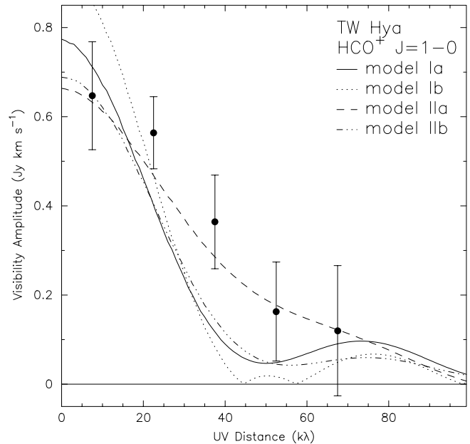
FIG. 5.—Visibility amplitude of observed and modeled \text{HCO}^+ J = 1-0 emission vs. baseline length, integrated over 0.5 km s ^{-1} width centered at LSR velocity 2.75 km s ^{-1} , annularly averaged in 15 k\lambda bins. The error bars represent \pm 1 standard deviation for each bin. The four curves show the visibility amplitudes derived from the model calculations of van Zadelhoff et al. (2001) that fit the single-dish observations of higher J \text{HCO}^+ transitions. Models Ia and Ib are based on the radiatively heated disk models of D’Alessio et al. (1999), and models IIa and IIb are based on the passive two-layer models of Chiang & Goldreich (1997). For model Ia (solid line) and model IIa (dashed line), \text{HCO}^+ is depleted by an overall factor of 100, with an additional order of magnitude drop when the temperature falls below 20 K. For model Ib (dotted line) and model IIb (dash-dotted line), \text{HCO}^+ emission is depleted by a factor of 500.
