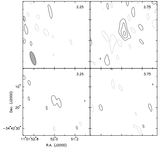
FIG. 2.—Velocity channel maps (width 0.5 km s ^{-1} ) of \text{HCO}^+ J = 1-0 line emission observed from TW Hya. The contour levels are \pm 2, 4, 6, \dots \times 66 mJy ( 0.7 K). Negative contours are dotted. The ellipse in the lower left corner of the upper left panel shows the 6''.9 \times 2''.1 P.A. 18^\circ synthesized beam.
