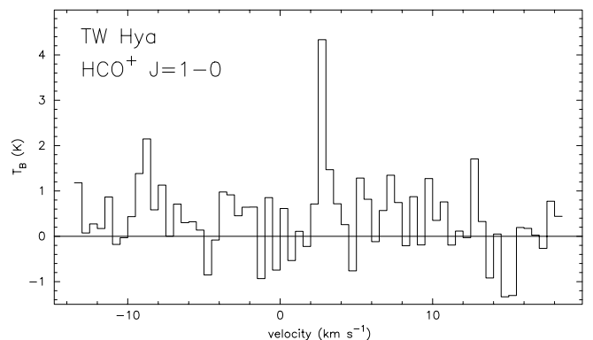
FIG. 3.—Spectrum of \text{HCO}^+ J = 1-0 line emission observed from TW Hya, at the position of peak continuum emission, binned to 0.5 km s ^{-1} velocity resolution, in the 6''.9 \times 2''.1 P.A. 18^\circ synthesized beam.
