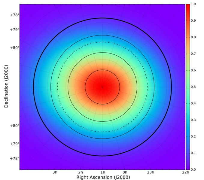
Figure 4. An example of a normalized PB map from one of the NCP observations, which has been scaled to 1.0. The bold, outer solid-line circle represents the full extent of the area for which the transient search was performed (radius of 7.5^\circ ). The inner solid-line circles show how the area was divided in order to gain an estimate of the average rms for each image accounting for the PB. The dashed-line circle indicates the position of the PB half-power point.
