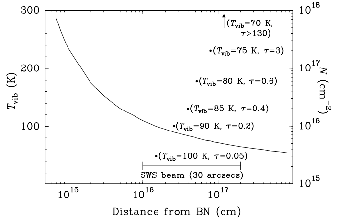
Fig. 8. Peak 1 vibrational excitation temperature (left axis) versus distance from BN for the physical model described in Sect. 4.2. The column densities of the best fitting models for CO 2 (right axis) are shown by the dots, assuming no background radiation, b = 10 km s -1 and a constant vibrational excitation temperature in the SWS beam as a function of radius. The x -coordinates of the dots refer to the radii at which the value of T_{\text{vib}} listed between parentheses occur. The optical depth of the most optically thick CO 2 ro-vibrational transition of the \nu_2 band is also listed. The position of the SWS beam w.r.t. BN is indicated.
