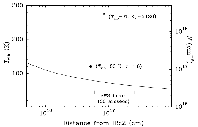
Fig. 9. Same as Fig. 8 but now for Peak 2. The source that is radiatively exciting the CO 2 molecules is the same as described in Sect. 4.2.
