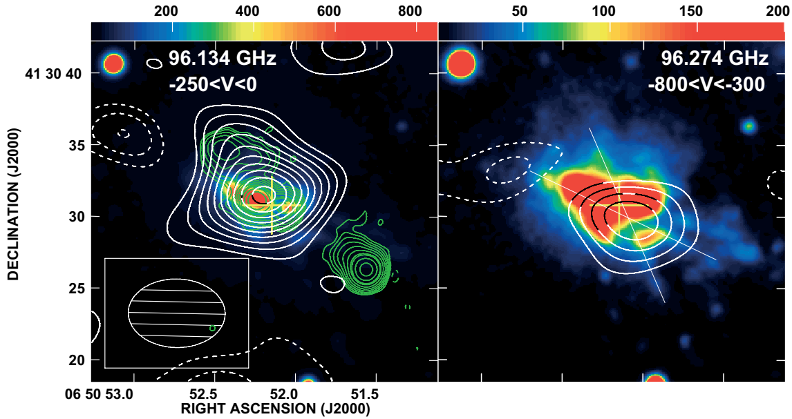
Fig. 3. Velocity-averaged CO maps (thick/white+black contours) of the red ( left ) and blue ( right ) components. CO contours are -3, -2, 3, \dots, 10\sigma , with \sigma = 0.2 \text{ mJy beam}^{-1} . The lower left inset shows the CO beam. The two CO maps are superposed on the \text{Ly}\alpha image, each with its own colour scheme to show the two dark lanes in the \text{Ly}\alpha . The thin green contours ( left panel ) show the 1.4 GHz radio map (Carilli et al. 1994), and the yellow cross indicates the radio core. The thin straight lines ( right panel ) indicate a possible AGN or starburst emission-line cone.
