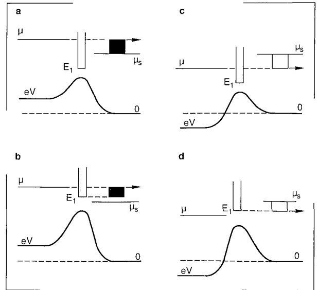
Fig 2 Schematic drawing of the injection of hot electrons over a point contact (in black) or of cool holes (in white) into the wide 2DEG region s. The local Fermi energies are denoted by \mu_1 and \mu_s in regions 1 and s respectively. The lowest 1D subband is indicated by the shaded column with subband bottom E_1 . The arrows denote the energy selected primarily in a differential focusing experiment.
