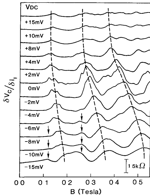
Fig 1 Electron focusing spectra dV_{34}/dI_{12} , for a range of applied DC bias voltages. The curves have been offset vertically for clarity. The dashed lines indicate the shift of the focusing peaks as a consequence of electron acceleration and deceleration over the point contact region. The arrows point to additional peaks observed for strong bias voltages.
