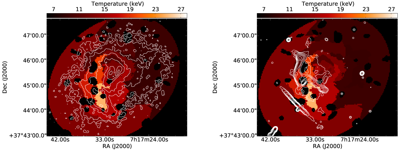
Figure 10. Temperature map of MACS J0717.5+3745. Overlaid are Chandra 0.5 – 4 keV surface brightness contours (left; based on the image in Figure 6) and JVLA radio contours (right; from Figure 3 middle panel). The X-ray contours are drawn at [0.013, 0.026, 0.052, 0.104, 0.208, 0.416, 0.832, 1.664] \times 10^{-6} photons \text{cm}^{-2} \text{s}^{-1} . The radio contours are drawn at [1, 2, 3, \dots] \times 4\sigma_{\text{rms}} .
