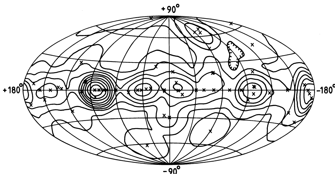
Figure 1: Approximate sky exposure achieved by the COS-B experiment. The contour levels are in 32 d steps, the lowest being 8 d (the exposure time is weighted with the inclination dependance of the sensitivity). The crosses indicate the pointing directions of the 65 observation periods.
