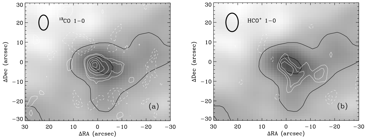
FIG. 4.—Integrated (a) OVRO ^{13}\text{CO} 1–0 and (b) \text{HCO}^+ 1–0 emission in the Elias 29 region ( white contours ) superposed on the 1.3 mm continuum map ( gray scale and black contours ). Contour levels are drawn at -3, -2, 2, 3, 6, \dots, 15 and -3, -2, 2, 3 , and 4 times the noise level ( 0.48 and 0.90 \text{Jy beam}^{-1} for ^{13}\text{CO} 1–0 and \text{HCO}^+ 1–0, respectively). The contours for negative signals are given by white dashed lines. Contour levels for the 1.3 mm map are the same as in Fig. 1. The synthesized OVRO beam size is given in the top left-hand corners.
