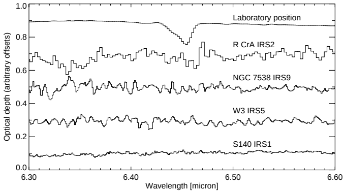
Fig. 1. ISO-SWS spectra of R CrA IRS2, NGC 7538 IRS9, W3 IRS5 and S140 IRS1 between 6.3 and 6.6 \mu\text{m} compared to that of solid O 2 in the laboratory, whose fundamental transition falls at 6.45 \mu\text{m} .
