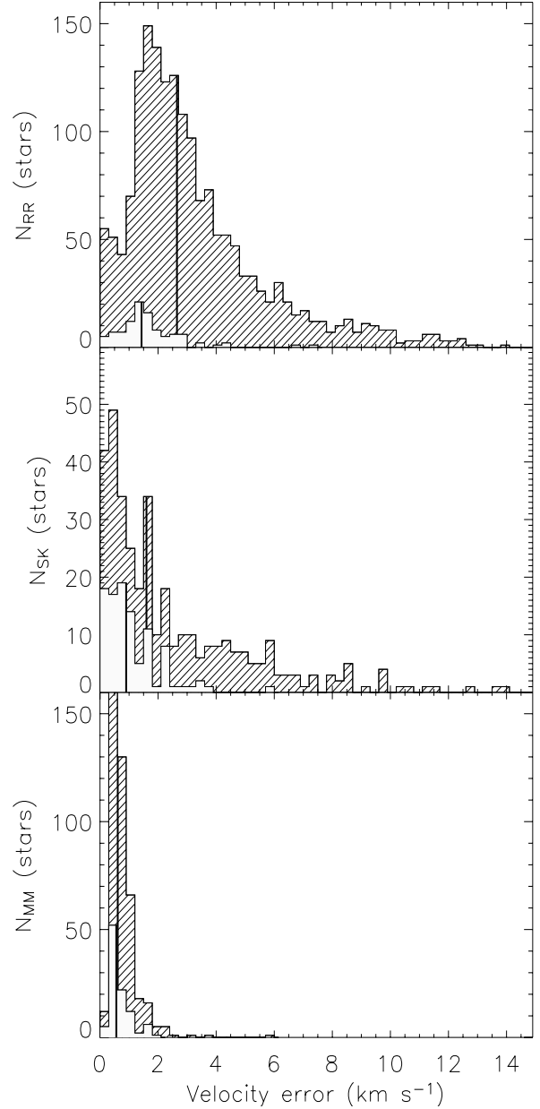
Fig. 2. Histograms of errors in the radial velocities reported for the rr , sk and mm samples (top, middle and bottom panel). The light-shaded areas are the similar histograms for the 93 stars in common between the three studies. The solid vertical lines indicate the median value of each of the distributions.
