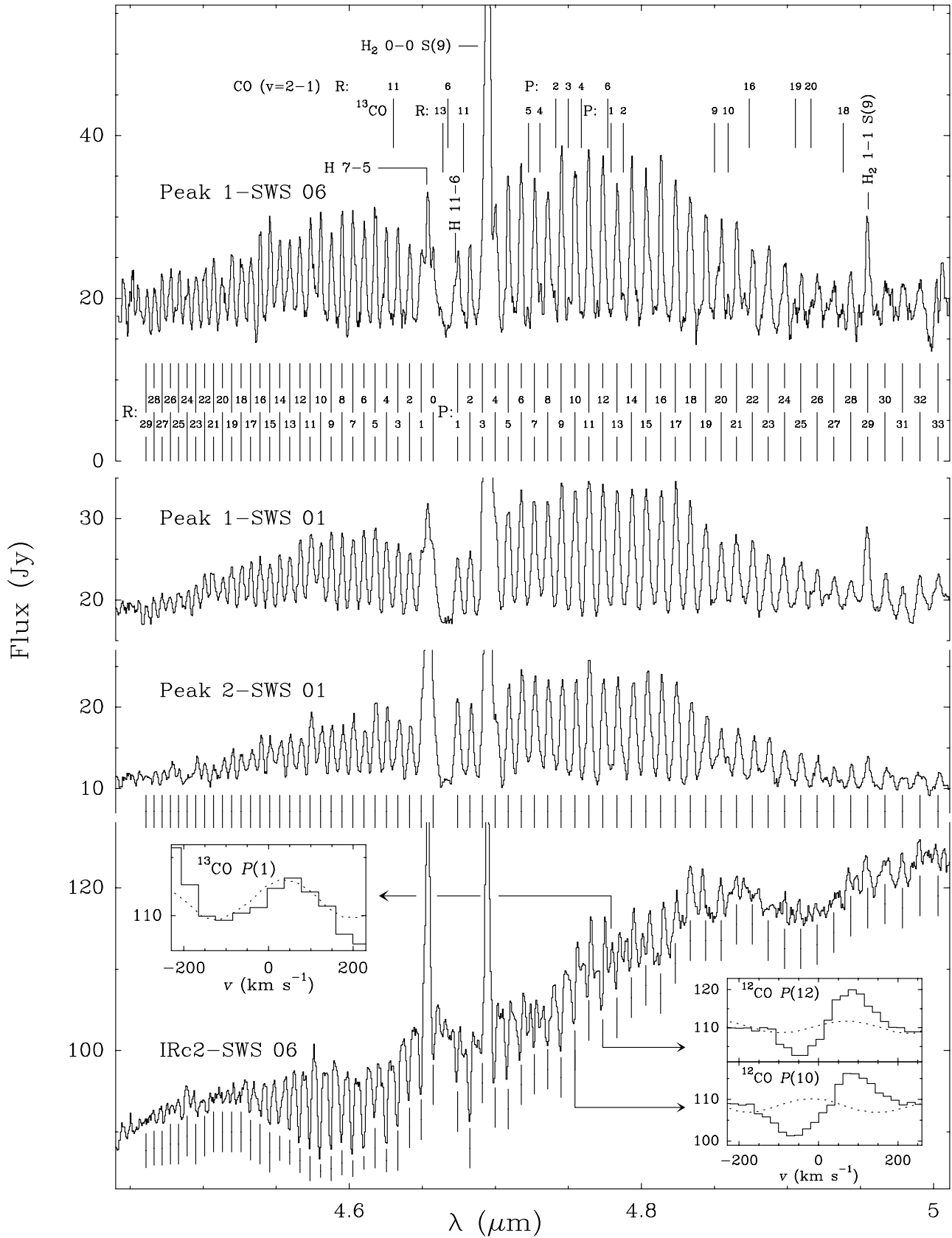
Fig. 1. Observed CO v = 1-0 band toward Orion/Peak 1 (SWS06 and 01 modes), Peak 2 (SWS01) and IRc2 (SWS06). In addition to the expected positions of the ^{12}\text{CO} v = 1-0 P(J) and R(J) lines, H 2 and HI lines, the positions of some ^{12}\text{CO} v = 2-1 and ^{13}\text{CO} v = 1-0 lines that are not coincident with any CO v = 1-0 line are also indicated in the upper spectrum. Insert panels show in more detail some profiles observed toward IRc2, and dashed lines indicate the RSRF scaled to the IRc2 continuum. The apparent ^{13}\text{CO} P(1) line is an effect of fringes.
