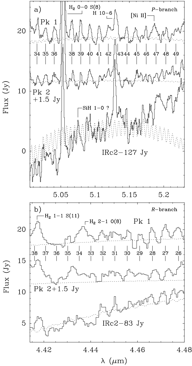
Fig. 2. Spectra around 5.12 and 4.45 \mu\text{m} observed towards Orion/Peak 1, Peak 2, and IRc2. The expected positions of the high- J CO v = 1-0 lines are labelled. Dashed lines indicate the expected RSRF scaled to the observed continuum.
