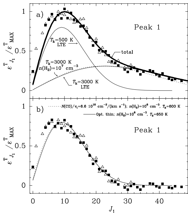
Fig. 8. Same as Figs. 7a,b but for collisional pumping (Peak 1).
