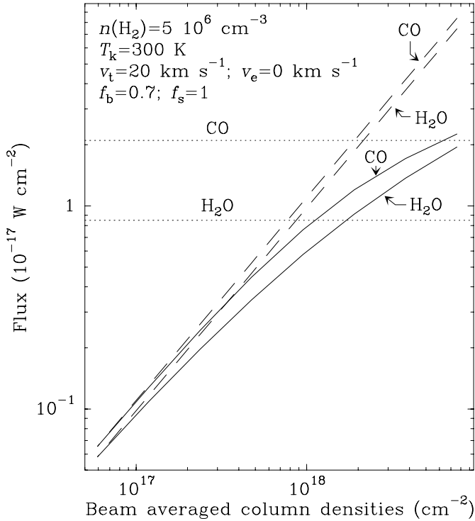
Fig. 13. CO v = 1-0 and H 2 O \nu_2 = 1-0 total fluxes versus beam-averaged column densities. Solid lines display the results of models that include opacity effects (Sect. 4.2.4). The solid angle subtended by the source is equal to that of the ISO/SWS beam ( f_b = 0.7 ; see text). Dashed lines indicate the linear relationship that would hold if the ro-vibrational lines were optically thin. Horizontal dotted lines indicate the observed fluxes from the warm component toward Peak 1 (values for Peak 2 are similar).
