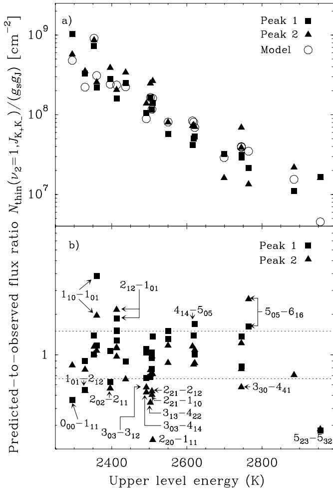
Fig. 19. a) H 2 O upper level column densities toward Orion/Peak 1 (squares) and Peak 2 (triangles), compared with the model prediction of Fig. 17e (circles). Column densities have been calculated from Eq. (2) (i.e., as proportional to the line fluxes) and by using the same lines for the observations and the model. b) Predicted-to-observed flux ratios. Dotted lines indicate values of 0.66 and 1.5.
