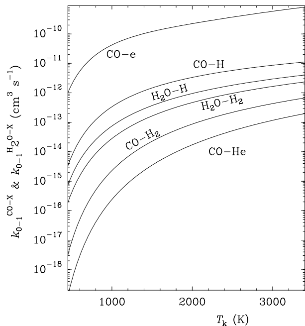
Fig. 9. Rate coefficients for CO v = 0-1 excitation through collisions with electrons, atomic hydrogen, molecular hydrogen, and helium, and for H 2 O \nu_2 = 0-1 excitation through collisions with atomic and molecular hydrogen. CO curves show fits to experimental data, and are reported by Draine & Roberge (1984) for CO-e, Glass & Kironde (1982) for CO-H, and Millikan & White (1963) for CO-H 2 and CO-He. H 2 O curves are based in Eq. (13).
