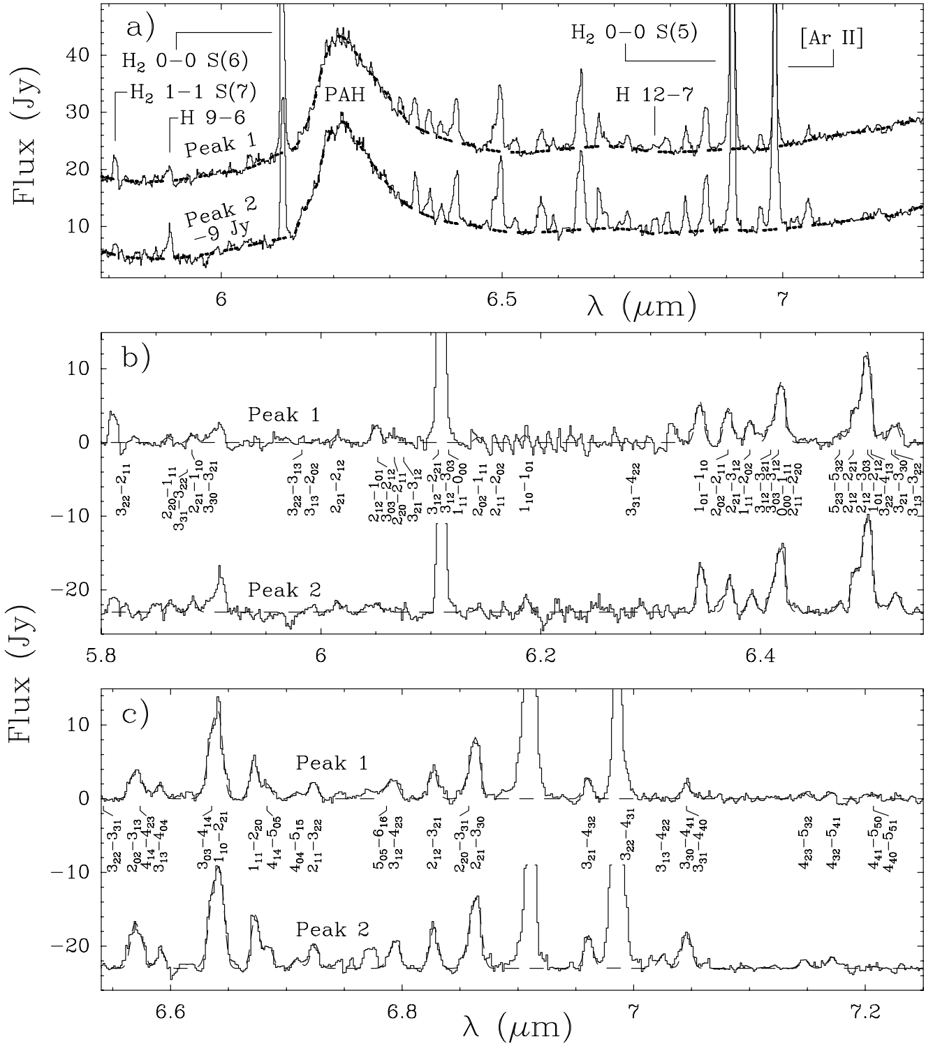
Fig. 5. a) Observed 5.8–7.2 \mu\text{m} spectrum toward Orion/Peak 1 and Peak 2. The dashed lines indicate the adopted continuum emission. Panels b) and c) show the resulting spectra after subtracting the above continuum. The positions of some H 2 O \nu_2 = 1-0 ro-vibrational lines are indicated, and dashed lines show Gaussian fits to the spectral features coincident with H 2 O lines.
