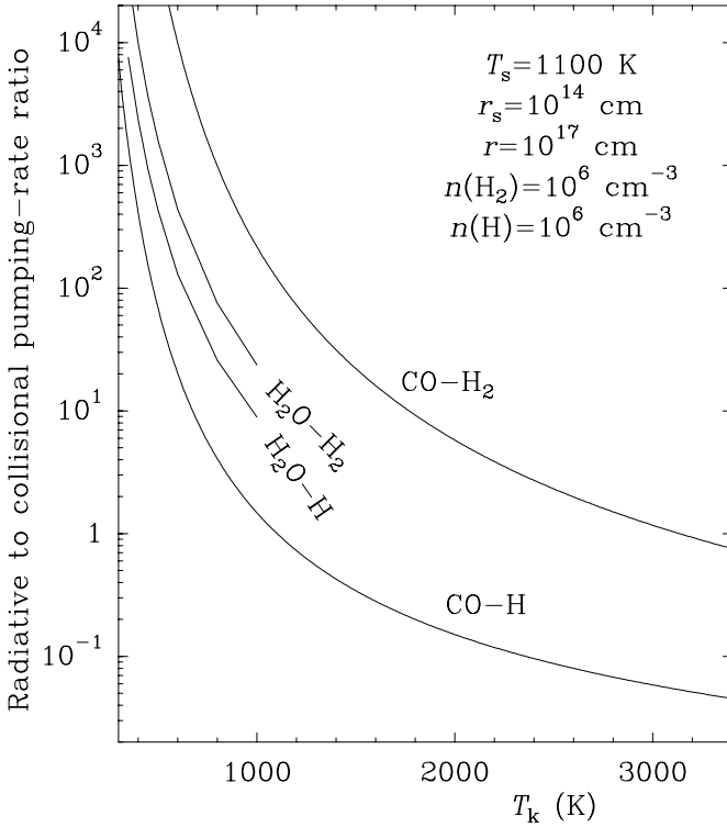
Fig. 10. Estimation of the radiative to collisional pumping rate ratio as a function of kinetic temperature. Rates of radiative excitation for CO have been computed from Eq. (6) (zero extinction is assumed) by summing over all v = 1 rotational levels, and similar expressions have been used for H 2 O. Molecules are assumed to be located at r = 10^{17} cm from the stellar source. Excitation through collisions with H 2 and H is considered, with assumed densities of 10^6 cm -3 for both cases.
