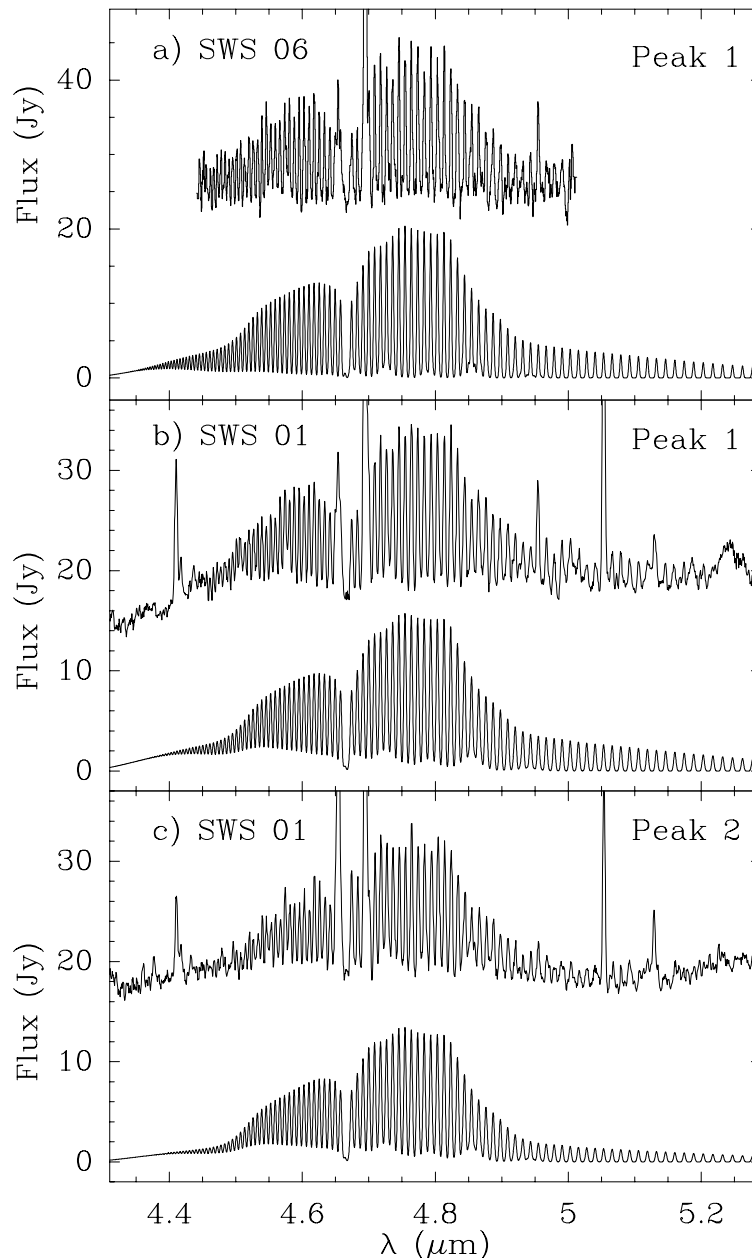
Fig. 16. Comparison between the observed CO v = 1-0 band and the composite hot-warm model prediction of Fig. 15d (after subtracting the continuum). An LTE T_k = 3 \times 10^3 K component has been assumed for the hot component, whereas the warm component includes ^{13}\text{CO} with an abundance 60 times lower than that of ^{12}\text{CO} . We have assumed \lambda/\Delta\lambda = \lambda/\Delta\lambda(4.7 \mu\text{m}) + 330(\lambda(\mu\text{m}) - 4.7) , where \lambda/\Delta\lambda(4.7 \mu\text{m}) = 1150 and 1500 in the SWS06 (panel a )) and SWS01 (panels b ) and c )), respectively. The model for the warm component at Peak 2 only differs from that of Fig. 15d in the fact that the illuminating flux has been reduced by 10%. The observed SWS06 spectrum of Peak 1 and SWS01 spectrum of Peak 2 have been shifted up 7 Jy and 8 Jy, respectively.
