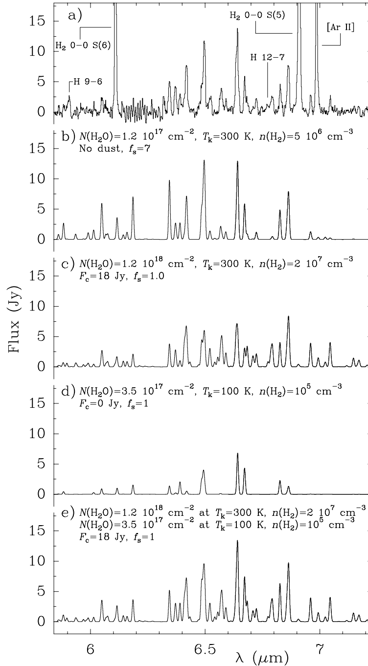
Fig. 17. Observed H 2 O ν 2 = 1-0 band toward Peak 1 a ) and model predictions b - e ). In all the models f_b = 0.7 , v_t = 20 \text{ km s}^{-1} , and v_e = 0 \text{ km s}^{-1} ; other varying parameters are indicated in the corresponding panels. In e ) the source is composed of the warm component in panel c ) (300 K) and the colder (100 K) component in panel d ).
