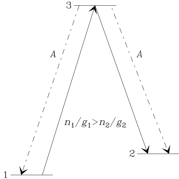
Fig. 14. 3-level molecular system that generally accounts for the P - R -asymmetry. The v = 0 rotational levels 1 and 2 are connected with the excited vibrational level 3 through R - and P -transitions (dashed arrows), for which we assume similar Einstein coefficients. If the mean intensity is similar for both 3-1 and 3-2 transitions, the transfer of population 1-3-2 (solid arrows) will take place as long as the population per magnetic sublevel is larger for level 1 than for level 2.
