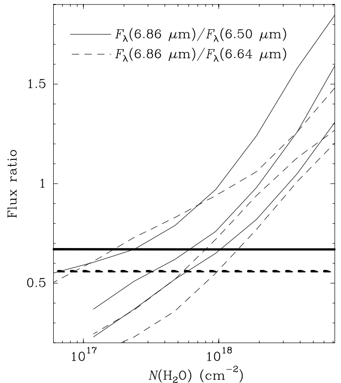
Fig. 18. Predicted flux ratio relation for the 6.86 \mu\text{m} to 6.5 \mu\text{m} spectral features (solid lines), and for the 6.86 \mu\text{m} to the 6.64 \mu\text{m} spectral features (dashed lines), versus beam-averaged H 2 O column density. The 6.86 \mu\text{m} feature corresponds to the joint emission of the H 2 O \nu_2 = 1\text{--}0 2_{21} \rightarrow 3_{30} and the 2_{20} \rightarrow 3_{31} lines, the 6.5 \mu\text{m} feature is the joint emission of the H 2 O \nu_2 = 1\text{--}0 1_{01} \rightarrow 2_{12} and the 2_{12} \rightarrow 3_{03} lines, and the 6.64 \mu\text{m} feature is the joint emission of the H 2 O \nu_2 = 1\text{--}0 1_{10} \rightarrow 2_{21} and the 3_{03} \rightarrow 4_{14} lines. Upper lines: n(\text{H}_2) = 5 \times 10^6 \text{ cm}^{-3} , T_{\text{k}} = 300 K; middle lines: n(\text{H}_2) = 5 \times 10^5 \text{ cm}^{-3} , T_{\text{k}} = 150 K; lower lines: n(\text{H}_2) = 2.5 \times 10^5 \text{ cm}^{-3} , T_{\text{k}} = 100 K. For all the calculations f_{\text{s}} = 1 , f_{\text{b}} = 0.7 , v_{\text{t}} = 20 \text{ km s}^{-1} , v_{\text{e}} = 0 \text{ km s}^{-1} , and dust is not included. Horizontal thick lines indicate the observed values at Peak 1. Toward Peak 2, the observed values are 0.74 (solid line) and 0.71 (dashed line).
