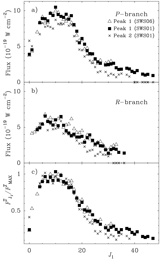
Fig. 3. CO v = 1-0 fluxes toward Peak 1 and Peak 2 in the a) P- and b) R-branches, determined from Peak 1/SWS06 data (triangles), Peak 1/SWS01 data (squares), and Peak 2/SWS01 data (crosses), plotted against the rotational quantum number J_1 of the upper v = 1 level. c) Normalized values of F_{J_1}^T \equiv F_{J_1}^P + F_{J_1}^R . We have adopted maximum fluxes of F_{\text{MAX}}^T = 1.6 \times 10^{-18} \text{ W cm}^{-2} for both SWS06 data (triangles) and SWS01 data (squares) of Peak 1, and F_{\text{MAX}}^T = 1.4 \times 10^{-18} \text{ W cm}^{-2} for the Peak 2/SWS01 data. For J_1 \geq 35 (Peak 1) or J_1 \geq 32 (Peak 2), F_{J_1}^R is calculated from F_{J_1}^P by correcting for the Einstein-A coefficient and frequency.
