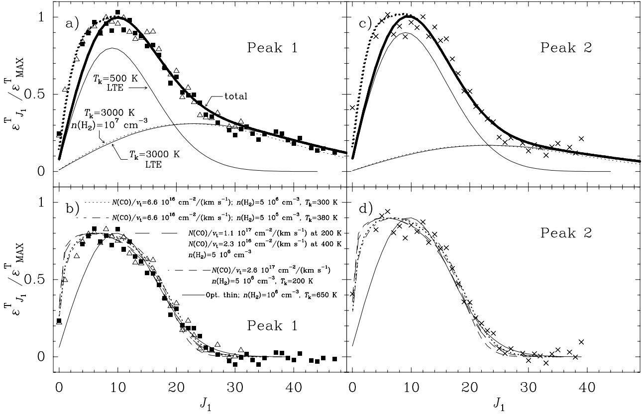
Fig. 7. Predicted and observed J_1 -distributions (a) and (b): Peak 1; (c) and (d): Peak 2) of the total flux arising in the P - and R -lines that have a common ( v = 1, J_1 ) level. Symbols have the same meaning as in Fig. 3. (a) and (c) Solid thin lines show results for the warm and hot components in the optically thin limit and assuming LTE. The distribution of the total flux, calculated by adding the fluxes from both T_k -components, is indicated by the solid thick line. The dashed thick line is the result of including a third (cold) T_k = 50 K component to match the flux of the low- J_1 lines. The dotted thin line displays the expected distribution in NLTE for the hot component by assuming n(\text{H}_2) = 10^7 \text{ cm}^{-3} . (b) and (d) Observed distribution after subtracting the predicted fluxes of the hot component (solid thin line in panel a for T_k = 3000 K). The different curves show the predicted distributions in NLTE for various labelled physical conditions (see text for details).
