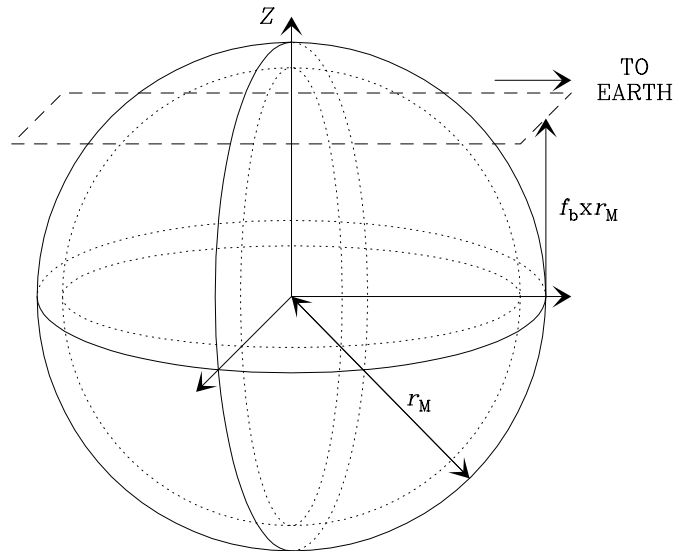
Fig. 12. Schematic representation of the modelled source, which is a spherical shell of gas with outer radius r_M = 2.1 \times 10^{17} cm and inner radius of r = 2 \times 10^{17} cm. Only the emission from the spherical cocoon above the dashed horizontal plane (with z coordinate f_b \times r_M ) is observed with the ISO/SWS beam. The column density calculated along the direction of the observer and averaged over this cocoon defines the beam-averaged column density.
