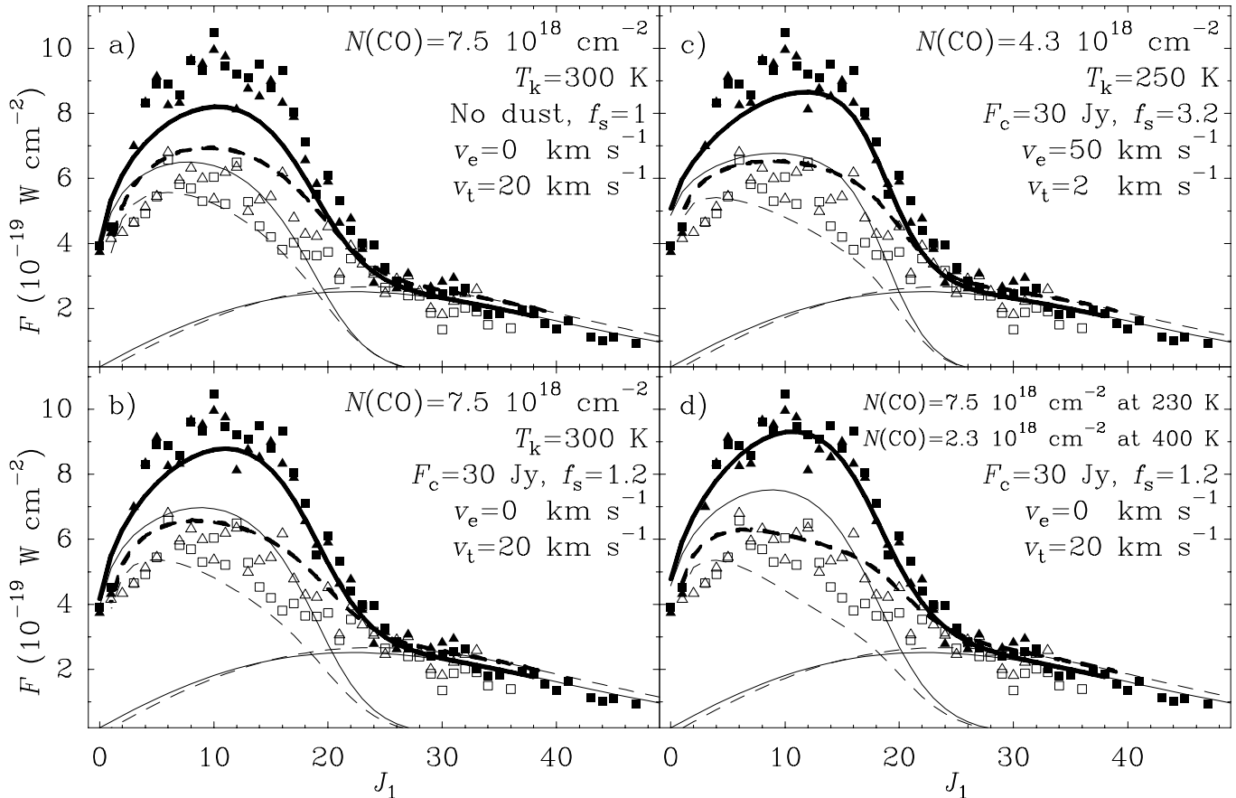
Fig. 15. CO v = 1-0 fluxes toward Peak 1 in the P - (filled symbols) and R - (open symbols) branches compared with model predictions. Triangles and squares indicate SWS06 and SWS01 data, respectively. Solid and dashed lines show results for the P - and R -branch, respectively. Thin lines show predictions for the hot ( 3 \times 10^3 K with v = 0 level populations in LTE) and warm (see text for details) components, and thick lines show the sum of both. Beam averaged CO column density, kinetic temperature, continuum flux, f_s factor, expansion velocity ( v_e ), and microturbulent velocity ( v_t ) used for the warm component are indicated in the corresponding panels.
