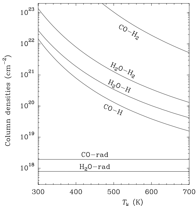
Fig. 11. Beam averaged CO and H 2 O column densities required to explain the observed fluxes toward Peak 1 from the warm component through collisions with H 2 (CO-H 2 and H 2 O-H 2 curves), collisions with H (CO-H and H 2 O-H), and resonant scattering (CO-rad and H 2 O-rad). Densities of 10^6 \text{ cm}^{-3} have been assumed for both H 2 and H. Calculations for resonant scattering assume that the ro-vibrational lines are optically thin, and the parameters T_s , r_s , and r are those of Fig. 10. Since band fluxes are very similar at both peaks, these results can be also applied to Peak 2.
