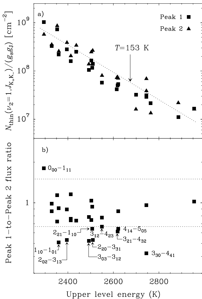
Fig. 6. a) Column densities of the H 2 O \nu_2=1 levels (squares: Peak 1; triangles: Peak 2), divided by the level degeneracy ( g_s = 3 for ortho-levels and 1 to para-levels; g_J = 2J + 1 ), plotted against the upper level energy. Column densities are computed in the optically thin limit. b) Peak 1 to Peak 2 line flux ratios. Only those lines with fluxes larger than 6 \times 10^{-20} \text{ W cm}^{-2} toward both peaks are accounted for. Lines are labelled when fluxes at both peaks differ in more than 50%, i.e. when the corresponding flux ratio lies out from the region between the dotted lines.
