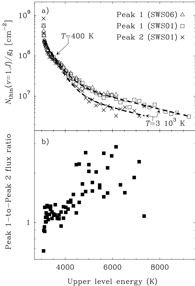
Fig. 4. a) Column densities of the CO v = 1 levels divided by the level degeneracy ( g_J = 2J + 1 ), plotted against the upper level energy. Column densities are computed in the optically thin limit. b) Peak 1 to Peak 2 line flux ratios.
