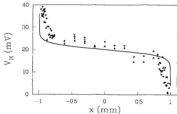
FIG. 2. Results of two line scans of the potential at magnetic fields of 5.0 T ( \blacktriangle ) and 5.25 T ( + ). The solid line is the result of a model calculation.
