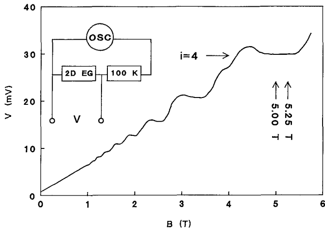
FIG. 1. Plot of the voltage across the sample vs magnetic field at a current of 5\text{ }\mu\text{A}_{\text{eff}} . The two-point experiment shows both plateaus and Shubnikov-de Haas oscillations. The arrows indicate the magnetic field at which line scans of the potential are made.
