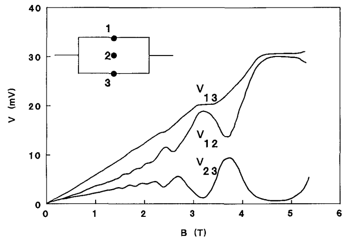
FIG. 3. Hall potential measurement as a function of B between the contacts indicated. Contrary to the results of the Pockels experiment, the current distribution seems to depend strongly on the magnitude of B in this case.
