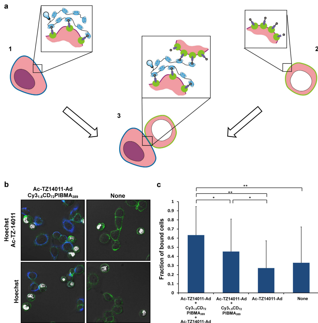
Figure 5. (a) Schematic overview of inducing cell-cell interactions (3) between \beta -CD polymer ( \text{Cy3}_{1.5}\text{CD}_{10}\text{PIBMA}_{389} ) functionalized cells (1) and Ad (Ac-TZ14011-Ad) functionalized cells (2) with Hoechst staining (white) (b) Representative confocal images of inducing supramolecular cell-cell interactions between variable functionalized MDAMB231 \times 4 cells. With GFP in green, Cy3 in blue and Hoechst in white. (c) Average values of the fraction of cell-cell interactions in each test condition. Significance of differences is marked with * ( p < 0.05 ) or ** ( p < 0.01 ).
