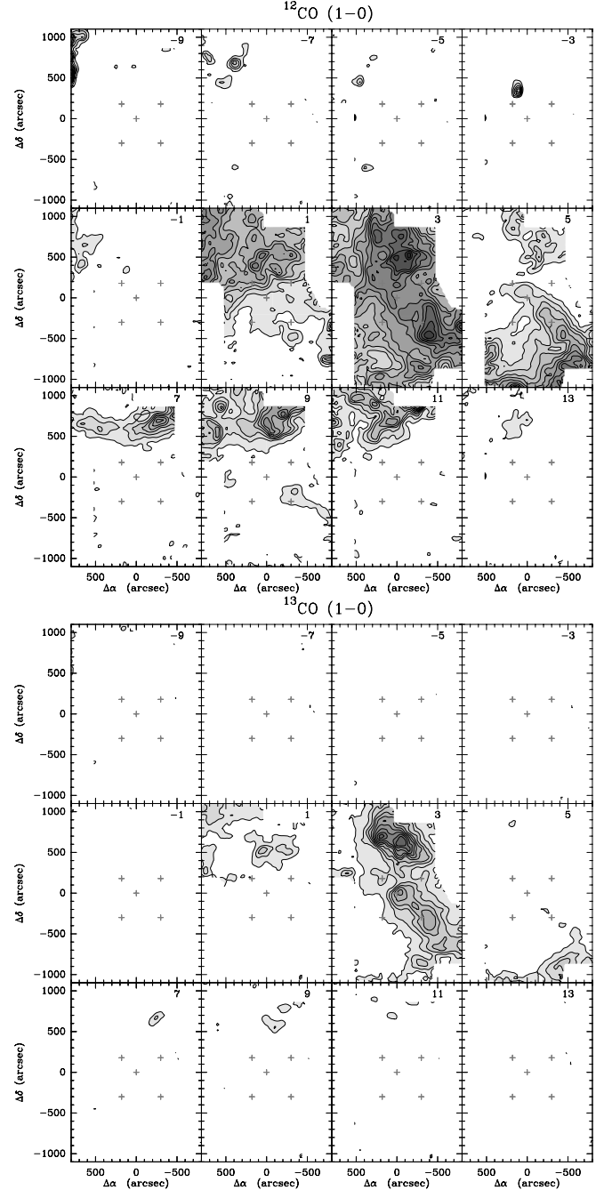
Fig. 6. Channel maps of the \text{CO}(1-0) (top panel) and ^{13}\text{CO}(1-0) (bottom panel) lines around the rest velocity of L1014. First contour and contour spacing are 0.8 \text{ K km s}^{-1} for the \text{CO} data and 0.05 \text{ K km s}^{-1} for the ^{13}\text{CO} ones. Velocity bins are spaced at 2 \text{ km s}^{-1} intervals and the starting velocity of the bin is reported in the top right corner of each map. The central cross on each map indicates the dust peak, while the other four delineate the area shown in Fig. 2.
