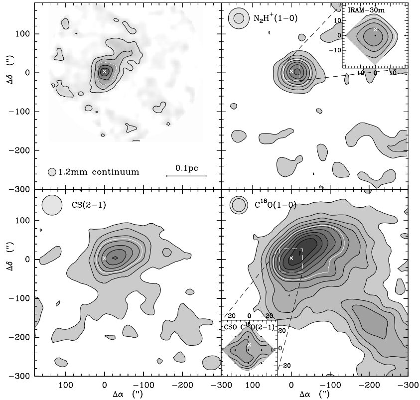
Fig. 2. 1.2-mm continuum, \text{N}_2\text{H}^+(1-0) , \text{CS}(2-1) and \text{C}^{18}\text{O}(1-0) emission towards L1014. Molecular line maps were taken at FCRAO with the exception of the \text{N}_2\text{H}^+(1-0) map in the inset (from IRAM-30 m) and the \text{C}^{18}\text{O}(2-1) map in the inset (from CSO). The 1.2-mm continuum was taken from Young et al. (2004) and it was observed with IRAM-30 m. First contour and contour spacings are 0.08 \text{ K km s}^{-1} for the FCRAO molecular data and 4 \text{ mJy}/(11'' \text{ beam})^{-1} for the dust continuum. The white contour represents the half peak intensity in all the maps. Beam sizes are displayed at the top-left of each map in all but the 1.2-mm map. The white cross places the position of a point-like source detected by the Spitzer Space Telescope, and colors are compatible with an embedded protostar. Angular offsets are relative to the 1.2-mm continuum peak ( 21^{\text{h}}24^{\text{m}}07^{\text{s}}.5 , 49^{\circ}59'05'' , J2000). The inset on the \text{N}_2\text{H}^+(1-0) FCRAO map shows the 5-points observations of \text{N}_2\text{H}^+(1-0) at IRAM-30 m. Levels start at 0.8 \text{ K km s}^{-1} and increase by 0.3 \text{ K km s}^{-1} . The IRAM-30 m beam size is shown inside that of the FCRAO. Similarly, the inset in the \text{C}^{18}\text{O}(1-0) FCRAO map shows the 13-points map of \text{C}^{18}\text{O}(2-1) taken at CSO. Levels start at 0.35 \text{ K km s}^{-1} and increase by 0.1 \text{ K km s}^{-1} . The CSO beam size is shown inside that of the FCRAO.
