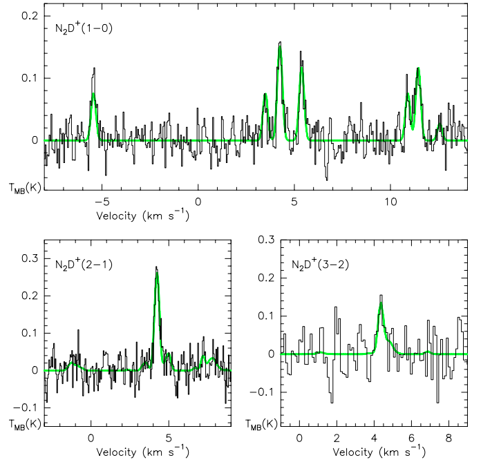
Fig. 4. \text{N}_2\text{H}^+ (1–0), \text{N}_2\text{H}^+ (3–2), \text{C}^{17}\text{O} (1–0), \text{N}_2\text{D}^+ (1–0), \text{N}_2\text{D}^+ (2–1), and \text{N}_2\text{D}^+ (3–2) spectra observed with the IRAM-30 m towards the 1.2-mm peak of L1014. Hyperfine fits are plotted.
