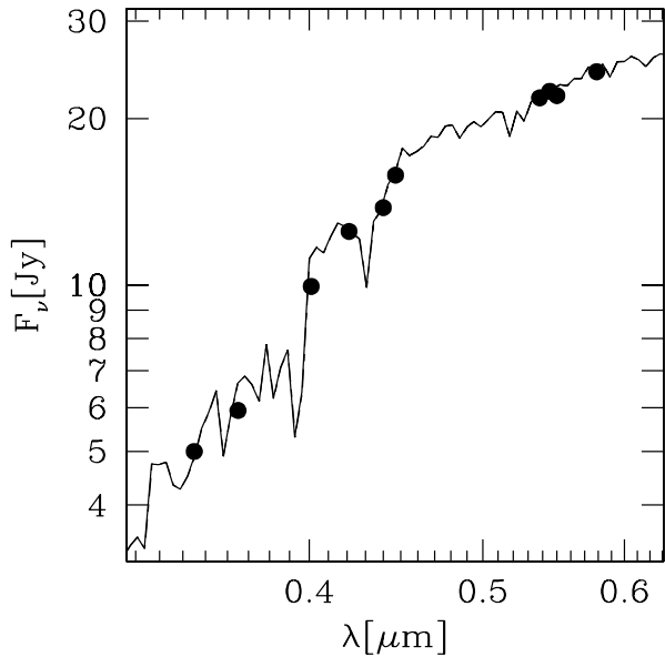
Fig. 1. The optical part of the Kurucz atmosphere fitted to the measured magnitudes of HD 207129. The big dots indicate magnitude measurements taken from the Geneva photometry catalogue (Rufener, 1988, 1989)
