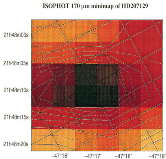
Fig. 2. ISOPHOT minimap of HD 207129 at 170 \mu\text{m} . Minimum flux at the edges of the map is about 5.5 \text{ MJy/sr} , and at the centre we detect a flux of 6.2 \text{ MJy/sr} .
