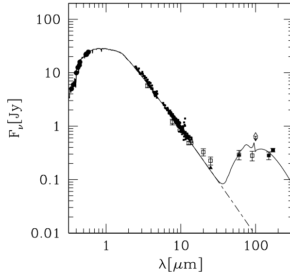
Fig. 4. Overview of the spectral energy distribution of HD 207129, with all measurements. Big dots indicate magnitude measurements taken from the Geneva photometry catalogue (Rufener, 1988, 1989). Small squares indicate measurements from PHT-S (filled squares) and CAM-CVF (open squares) spectra. Large squares indicate photometry with ISOPHOT P. Filled triangles are IRAS (IFSC data) and the open triangle is the 100 \mu\text{m} IRAS (IFSC) upper limit. The solid line shows the flux derived from the model using cometary dust grains (case B). The dashed line indicates the purely photospheric flux.
