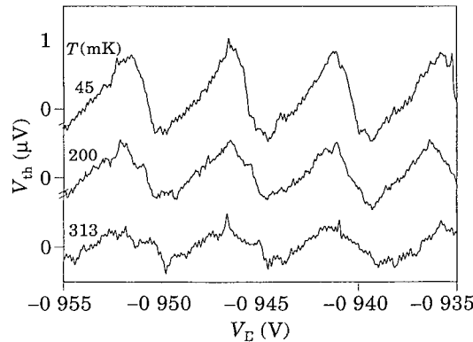
Fig. 3. – Thermovoltage V_{\text{th}} as a function of V_E at lattice temperatures of T = 45, 200 and 313 mK, obtained using a heating current of 18 nA.
