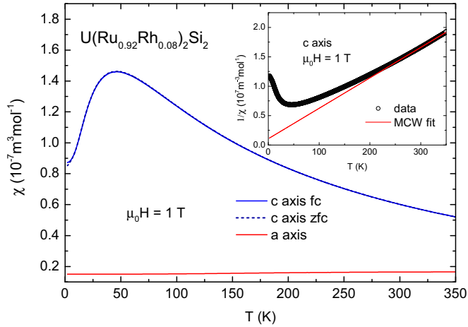
FIG. 3. Temperature dependence of the static magnetic susceptibility \chi = M/H of the unannealed \text{U(Ru}_{0.92}\text{Rh}_{0.08})_2\text{Si}_2 single crystal measured at 1 T applied along the principal axes. In the inset we show the temperature dependence of the inverse magnetic susceptibility measured in 1 T applied along the tetragonal axis together with the best fit to a Curie-Weiss law to data above 300 K.
