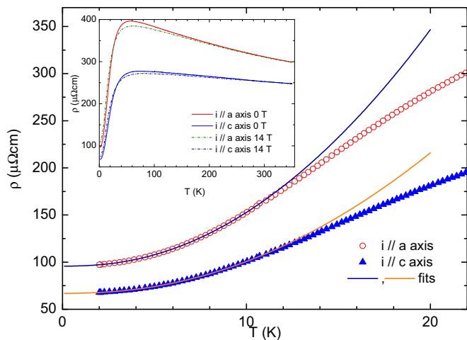
FIG. 6. The zero-field low-temperature dependence of the \text{U(Ru}_{0.92}\text{Rh}_{0.08})_2\text{Si}_2 electrical resistivity for current along the a and the c axis together with the best fit described in the main text. In the inset the electrical resistivity measured along the a axis and the c axis in the whole temperature range in zero field and 14 T applied along the tetragonal axis is shown.
