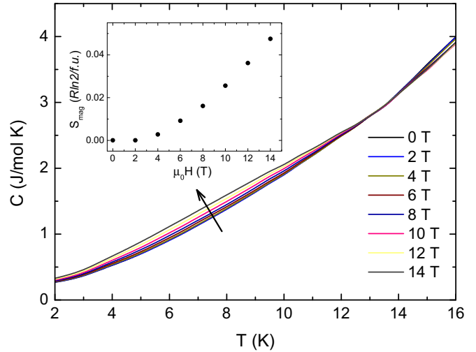
FIG. 10. The temperature dependences of the \text{U(Ru}_{0.92}\text{Rh}_{0.08})_2\text{Si}_2 specific heat measured at different magnetic fields applied along the tetragonal axis. In the inset the magnetic entropy calculated by integration of data shown in the main panel (from which an estimate of a nonmagnetic analog contribution has been subtracted) divided by the temperature up to 14 K is shown.
