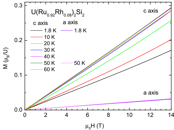
FIG. 5. Field dependence of the \text{U(Ru}_{0.92}\text{Rh}_{0.08})_2\text{Si}_2 single-crystal magnetization measured at various temperatures between 1.8 K and 60 K with field applied along the a and the c axis. Note the nearly linear M - H behavior throughout.
