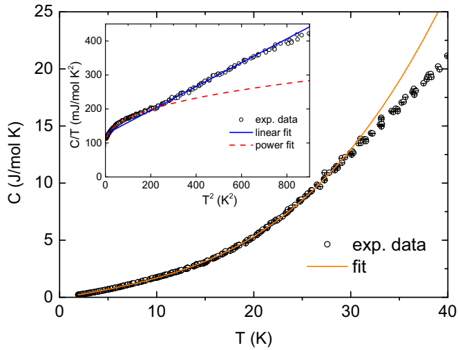
FIG. 9. The temperature dependence of the \text{U(Ru}_{0.92}\text{Rh}_{0.08})_2\text{Si}_2 specific heat together with the best fit containing an exponential term (see the main text). In the inset the low-temperature detail of the C/T vs T^2 dependence is shown along with the best fits to a linear (solid, blue line) and power-law (dashed, red line) dependencies, respectively.
