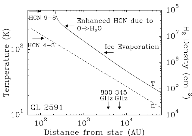
FIG. 2.—Temperature and density structure of GL 2591. The critical densities for the \nu_2 = 0 J = 9-8 and \nu_2 = 0 J = 4-3 lines are indicated as well as the JCMT beam sizes at the different frequencies (adapted from van Dishoeck & van der Tak 2000).
