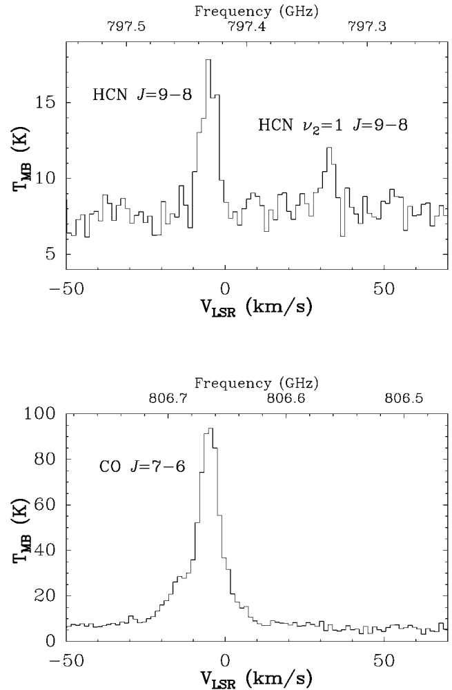
FIG. 1.— Top : Spectrum of the \nu_2 = 0 J = 9-8 and the vibrationally excited \nu_2 = 1 J = 9-8 line of HCN at 797.434 and 797.330 GHz, respectively, toward the massive protostar GL 2591. The spectrum has been smoothed to a spectral resolution of \sim 1.4 \text{ km s}^{-1} . Bottom : The CO J = 7-6 line at 806.652 GHz is shown for comparison. The latter spectrum shows clearly the presence of a wing component, whereas the HCN J = 9-8 lines do not show such a component. The vertical offset shows the submillimeter continuum due to warm dust, which agrees within 30% with the 350 \mu\text{m} continuum photometry of this source (van der Tak et al. 2000).
