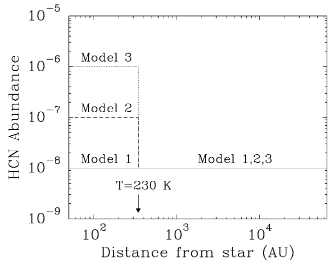
FIG. 3.—Different HCN abundance profiles used in the analysis of § 4 (see also Table 1).
