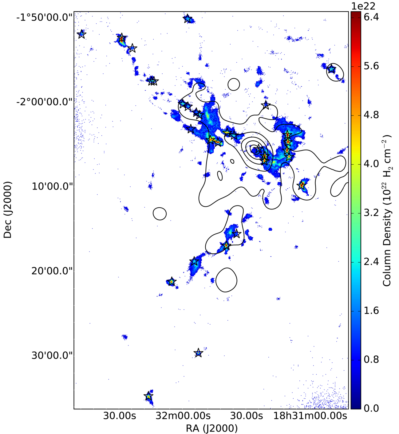
Figure 17. SCUBA-2 column density map of the W40 complex. Column density is shown for areas where emission is detected at or above S/N = 3 at 850 \mu\text{m} . Column density is calculated using temperatures as presented in Fig. 10 where available and a constant value of 15 K where a derived temperature is not. Contours describe YSO surface density with levels at 20, 60, 110, 160 and 210 YSO \text{pc}^2 . Stars mark the location of each dense core identified in Table 7.
