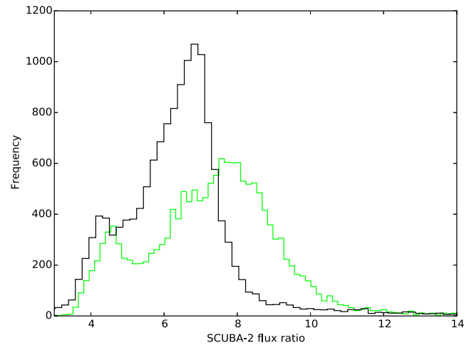
Figure 4. The distribution of 450 \mu m/850 \mu m flux ratio for the original (black) and CO-subtracted (light grey line, green in the online version) Aquila reductions with additional 4 arcmin spatial filtering. KS-statistics reveal a 1.3 per cent chance that the two data sets are drawn from the same distribution.
