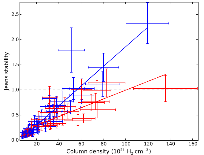
Figure 19. Jeans stability, M_{850}/M_J , as a function of column density. Exterior peripheral clumps (defined as having a mean Herschel 70 \mu\text{m} flux of less than 1000 MJy Sr -1 ) are marked in blue, interior clumps within the nebulosity Sh2-64 are marked in red. The unweighted linear regression fit to each population is marked as a line of the same colour.
