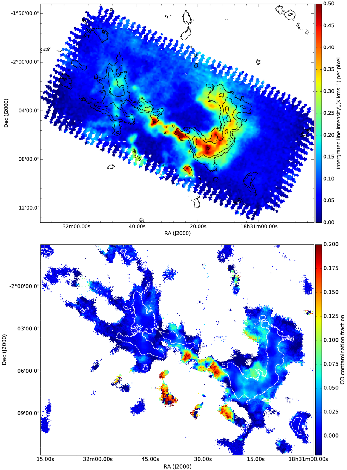
Figure 3. Upper: ^{12}\text{CO} 3–2 integrated intensity map over the entire range (from -90 to +100 \text{km s}^{-1} ) of the central region of the W40 complex. Contours show SCUBA-2 850 \mu\text{m} emission at the 5\sigma , 15\sigma and 50\sigma levels. Lower: the fraction of SCUBA-2 850 \mu\text{m} that can be attributed to ^{12}\text{CO} 3–2 345 GHz line emission. The SCUBA-2 data are masked at 3\sigma and the 5\sigma level is shown by the white contour.
