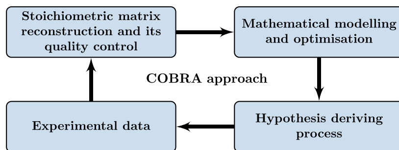
Fig. 1. Constraint-based reconstruction and analysis. Constraint-Based Reconstruction and Analysis (COBRA) is an example of a systems biology approach, carried out in an iterative cycle, where the aim is to increase the predictive accuracy of a constraint-based computational model. Quality controlled reconstruction of prior literature information generates a draft model, which includes a stoichiometric matrix (upper left). This is followed by mathematical modelling using optimisation methodologies (upper right), enabling hypothesis generation in the form of model predictions (lower right). These predictions are testing against experimental data (lower left) and any discrepancy is used to refine the reconstruction. This iterative cycle is repeated until a desired accuracy is reached.
