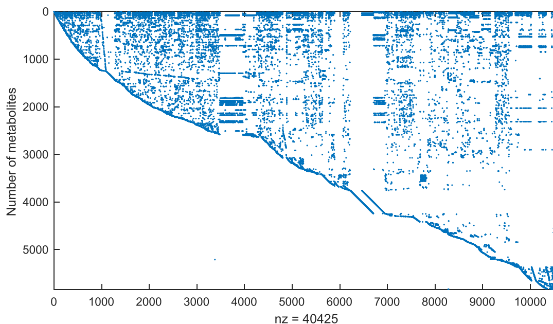
Fig. 8. The stoichiometric matrix of Recon3D. This stoichiometric matrix consists of 5835 rows (molecular species not molecules) and 10,600 columns (reactions). Only 0.065% (40, 425/61, 851, 000) of entries are non-zero (nz). The approximate upper diagonal appearance is due to the ordering of the reactions, rather than an intrinsic feature of a stoichiometric matrix. For genome-scale biochemical networks, stoichiometric matrices are sparse because molecular cardinality is typically less than 10 for most reactions.
