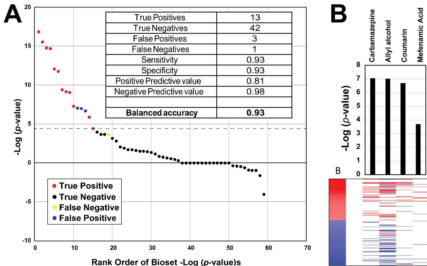
Fig 2. Predictive accuracy of the NRF2 biomarker. A. Predictions using the NRF2 biomarker were compared to those from the HTS NRF2 activation assays. The dashed line represents the cutoff value of four for significant biomarker activation. Those chemicals that were active (red) or inactive (black) in the HTS assays are shown. Three false positives (blue) and one false negative (yellow) are indicated. Inset, binary classifier calculations based on NRF2 HTS assay results. B. Expression changes of the biomarker genes for the three false positives and one false negative. (Top) The bar graph shows the -Log(p-values) of the comparisons between the biomarker and the indicated chemical. (Bottom) The heatmap shows the expression of the biomarker genes.
