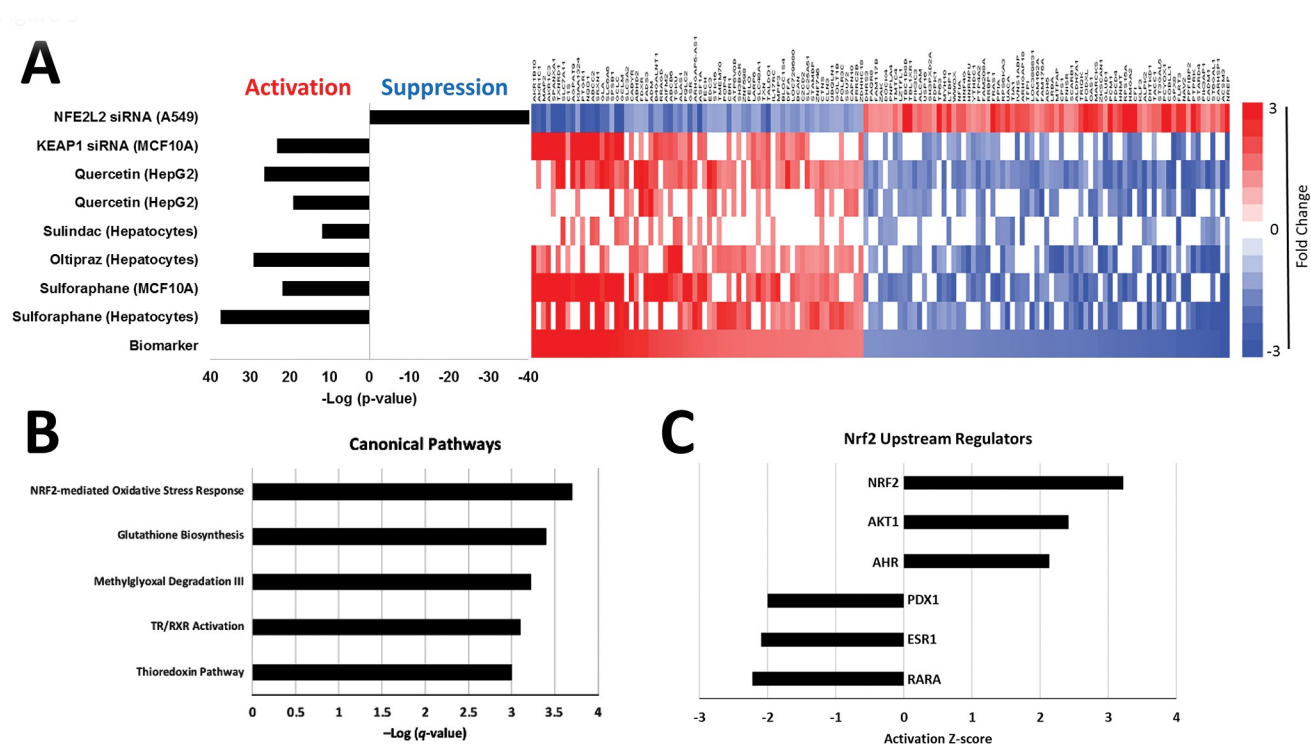
Fig 3. Characterization of the human NRF2 biomarker. A. Identification of NRF2 biomarker genes was based on consistent directional changes in gene expression resulting from exposure to NRF2 activators sulforaphane (GSE20479 and GSE28813), oltipraz (GSE20479), sulindac (TG-GATES), and quercetin (GSE28878), and knockdown of the NRF2 negative regulator Keap1 (GSE28813). Changes in gene expression were required to be in the opposing direction in cells in which NFE2L2 (NRF2) expression was knocked down (GSE38332). The bars on the left represent the -\text{Log}(\text{p-value}) for the Running Fisher comparison test between the biomarker and the individual biosets used to construct it. The heatmap on the right depicts gene expression changes for the 143 genes in the biomarker across the individual biosets. B. Canonical pathway analysis of the biomarker genes. Multiple test correction on p-values derived from the right-tailed Fisher's exact tests was carried out using the Benjamini-Hochberg method. The -\text{Log}(\text{q-value}) s are shown. C. Potential upstream regulators of NRF2 biomarker genes (activation z-scores > |2| ). Only upstream regulators with q-values < 0.05 are shown. Both analyses were conducted using Ingenuity Pathway Analysis software.
