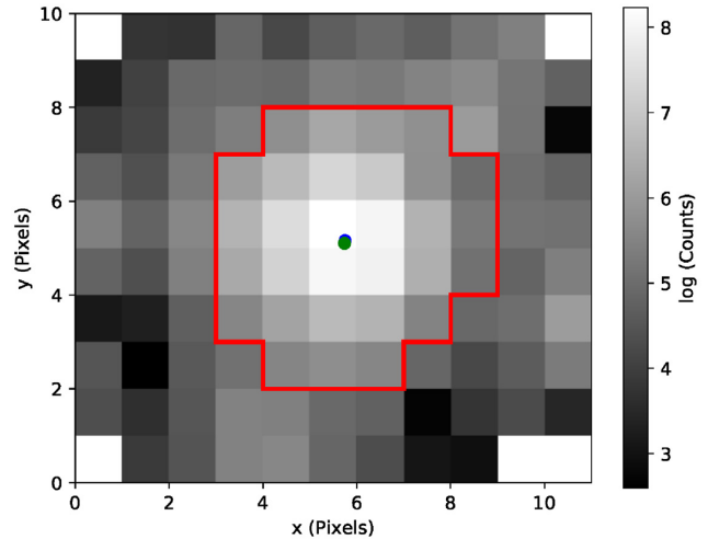
Figure 1. K2 image of K2-280 . Red lines show the aperture defined by the amount of light of each pixel and level of background light. The electron count is indicated by the intensity of shading (light grey for high and dark grey for low count). The green circle indicates the current position of the target in the EPIC catalogue, and the blue circle is the centre of the flux distribution. The scale of the image is the Kepler pixel scale of 3.98 \text{ arcsec pix}^{-1} . The K2 image is not a rectangle, but it is irregularly shaped. The white pixels in the corners contain no data.
