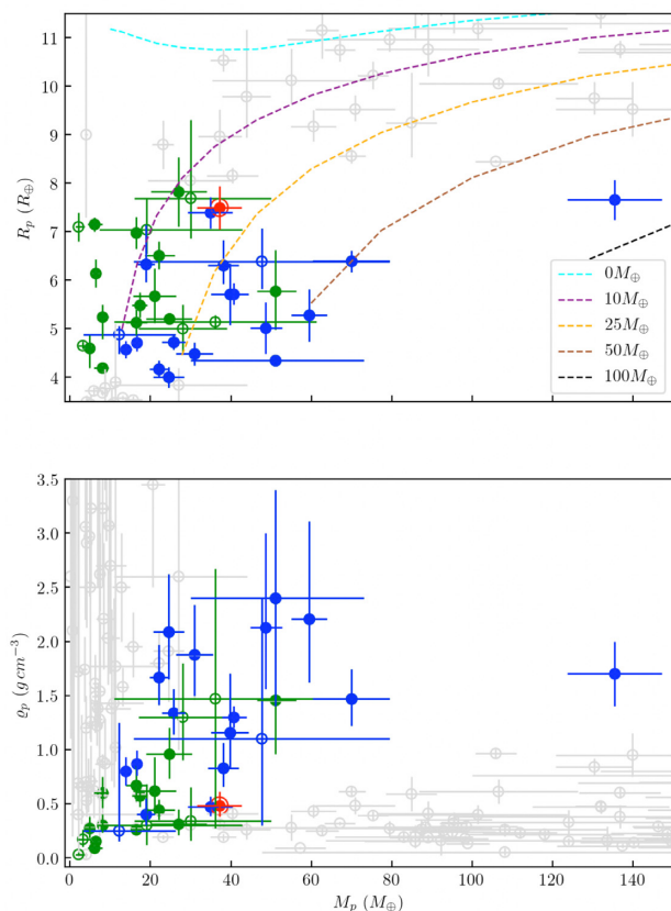
Figure 6. Mass–radius (upper panel) and mass–density (lower panel) diagrams for a sample of sub-Saturns ( R_p = 4\text{--}8 R_{\oplus} ). Sub-Saturns whose mean densities have been measured with a precision better than 50 per cent located in multiplanet systems are marked with green filled circles, whereas those in single systems are marked with blue filled circles. The position of K2-280 b is indicated as a red-rimmed circle. Sub-Saturns with densities measured with a precision slightly worse than 50 per cent are marked with green and blue open circles. The remaining planets with measured radii, masses, and mean densities (NASA Exoplanet Archive (Akeson et al. 2013), as of 2019 July) are marked with open grey circles. The dashed lines on the mass–radius diagram (upper panel) correspond to the Fortney et al. (2007) models for planet core masses of 0, 10, 25, 50, and 100 M_{\oplus} and age 10 Gyr.
