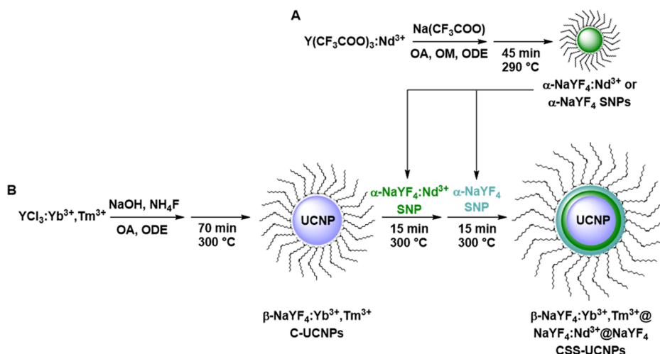
Scheme 2. Synthesis Schemes for the Preparation of (A) \alpha -NaYF 4 :Nd 3+ or \alpha -NaYF 4 SNPs and (B) \beta -NaYF 4 :Yb 3+ ,Tm 3+ @NaYF 4 :Nd 3+ @NaYF 4 CSS-UCNPs a
