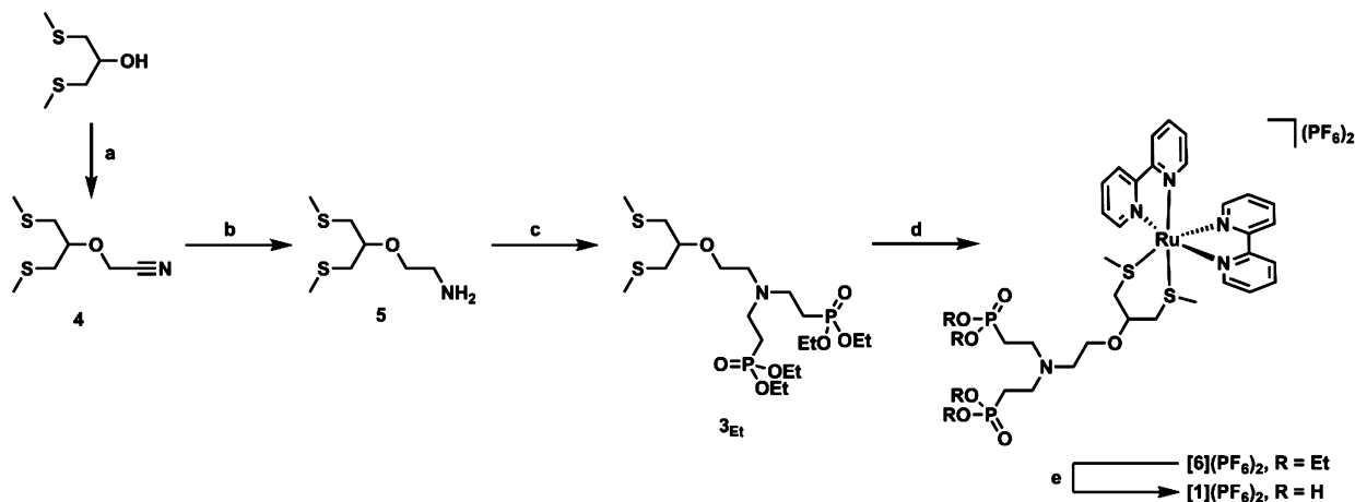
Scheme 3. Synthesis of the Ruthenium Complex [1](PF_6)_2^a
