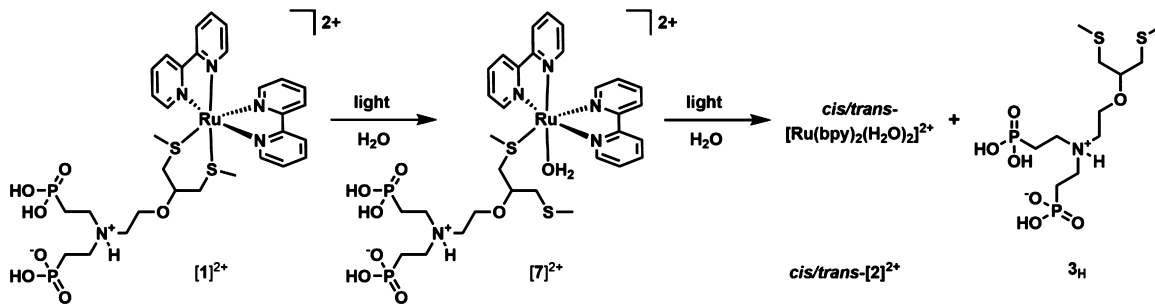
Scheme 4. Two-Step Photoreaction Observed upon Blue-Light Irradiation of a Solution of [1]^{2+} in H_2O
