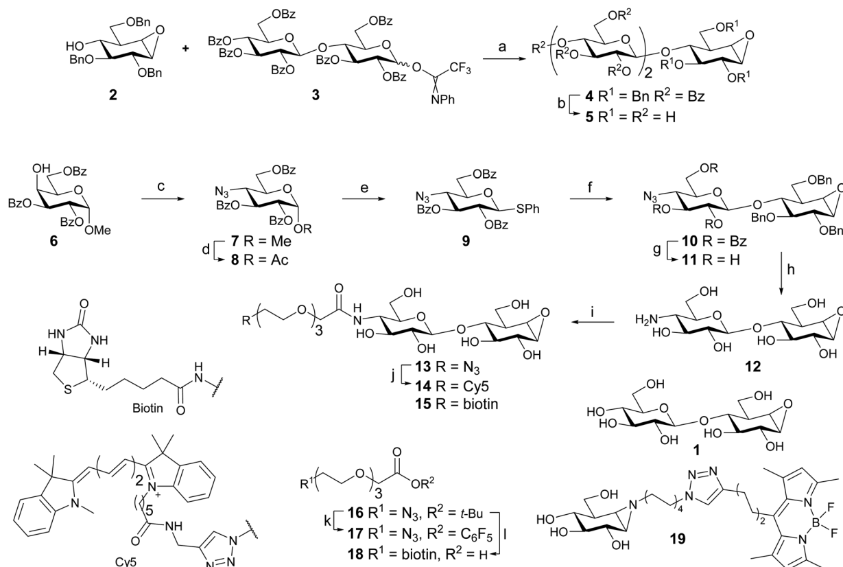
Scheme 1 Reagent and conditions: (a) TSMOTf, DCM, -15^{\circ}\text{C} to 0^{\circ}\text{C} , 45%. (b) (i) NaOMe, MeOH. (ii) \text{H}_2 , \text{Pd}(\text{OH})_2/\text{C} , \text{H}_2\text{O} , MeOH, dioxane, 40%. (c) (i) \text{TiF}_2\text{O} , pyr, DCM, -55^{\circ}\text{C} to rt. (ii) \text{NaN}_3 , DMF, 80^{\circ}\text{C} , 90%. (d) \text{Ac}_2\text{O} , AcOH, \text{H}_2\text{SO}_4 . (e) HSPH, \text{BF}_3\cdot\text{Et}_2\text{O} , DCM, 46% over 2 steps. (f) 2 , \text{Ph}_2\text{SO} , \text{TiF}_2\text{O} , TTBP, DCM, -70^{\circ}\text{C} to rt, 64%. (g) NaOMe, MeOH, DCM, 60%. (h) Na (s), t\text{-BuOH} , \text{NH}_3 , -60^{\circ}\text{C} , 53%. (i) 17 , DIPEA, DMF, 27%; or 18 , PFPOH, DIC, \text{Et}_3\text{N} , DMF, 44%. (j) Cy5 alkyne, THPTA, CuI, DIPEA, DMSO, 46%. (k) (i) TFA, DCM; (ii) PFPOH, DIC, DMAP, DCM, 67%. (l) (i) \text{PPh}_3 , \text{H}_2\text{O} , THF, 88%; (ii) BiotinNHS, DIPEA, DMF, 83%; (iii) TFA, DCM, quant.
