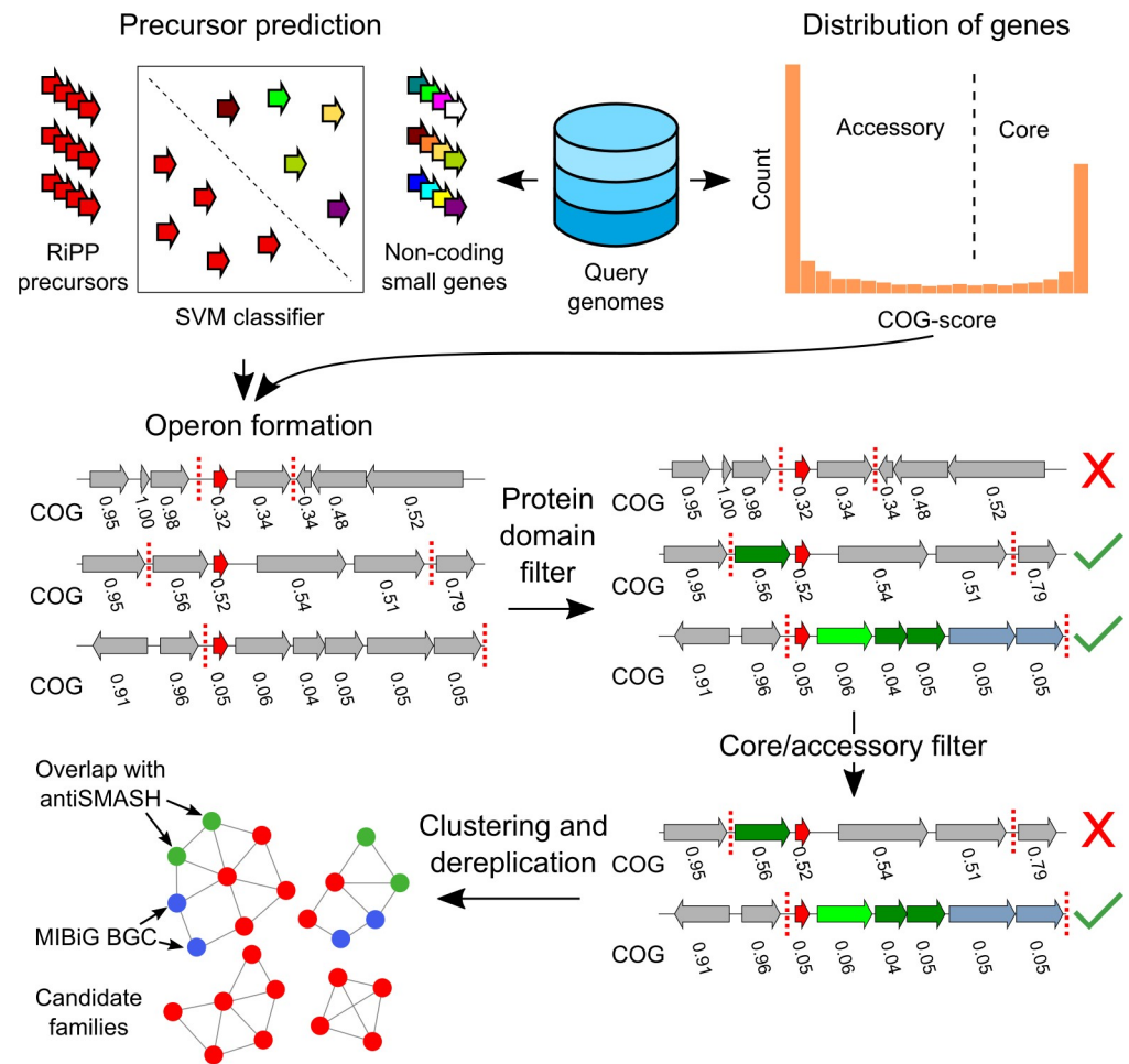
Fig 1. decRiPPter pipeline for the detection of novel RiPP families. The SVM classifiers is used to identify all candidate RiPP precursors in a given group of genomes, using all predicted proteins smaller than 100 amino acids. The gene clusters formed around the precursors are analyzed for specific protein domains. In addition, all COG scores are calculated to act as an additional filter and to aid in gene cluster detection. The remaining gene clusters are clustered together and with MIBiG gene clusters to dereplicate and organize the results. In addition, overlap with antiSMASH detected BGCs is analyzed. BGC, biosynthetic gene cluster; COG, cluster of orthologous genes; decRiPPter, Data-driven Exploratory Class-independent RiPP Tracker; MIBiG, Minimum Information about a Biosynthetic Gene cluster; RiPP, ribosomally synthesized and post-translationally modified peptide; SVM, Support Vector Machine.
