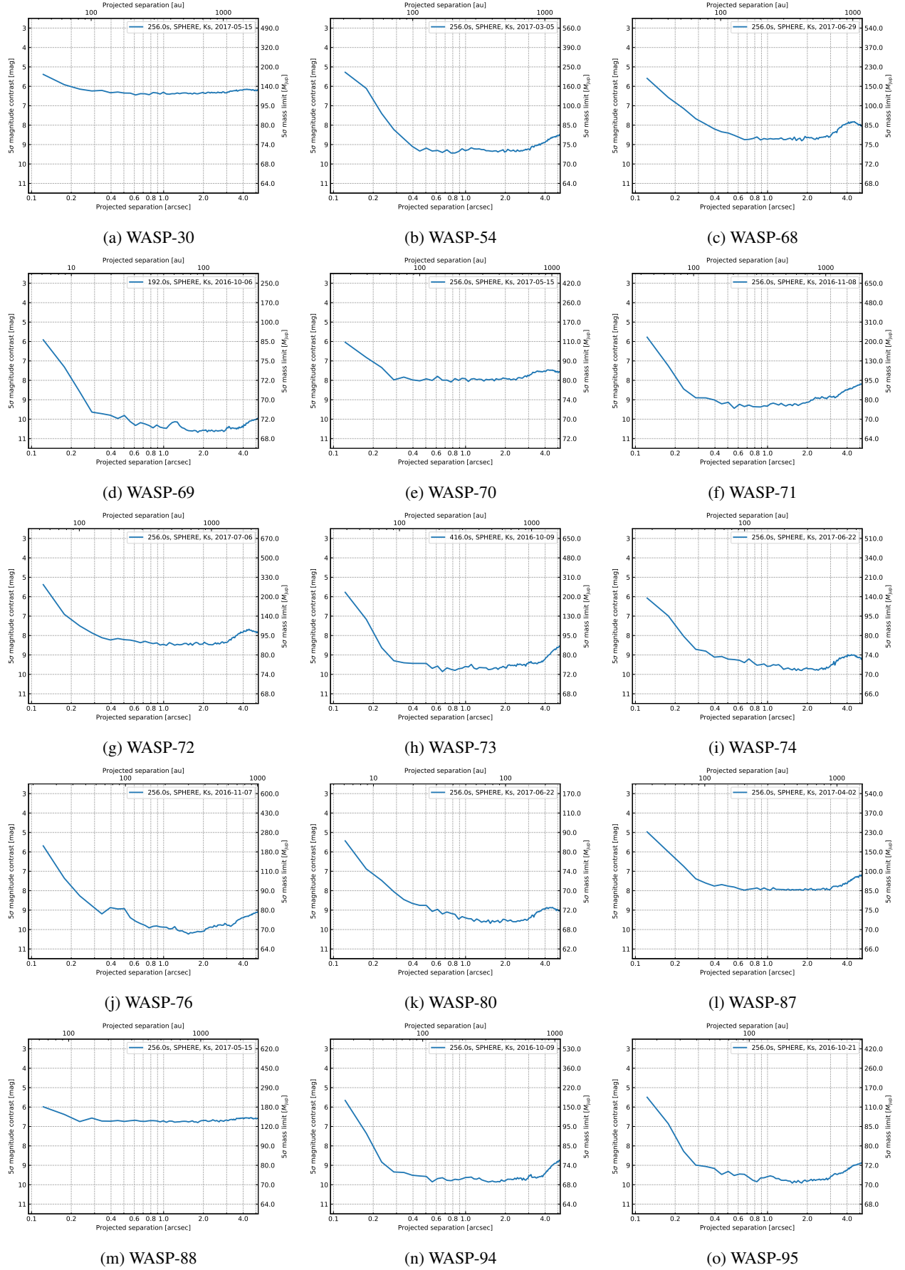
Fig. A.2: Detection limits of individual targets II. We convert projected angular separations in projected physical separations by using the distances presented in Table 1. The mass limits arise from comparison to AMES-Cond, AMES-Dusty, and BT-Settl models as described in Sect. 4.2.
