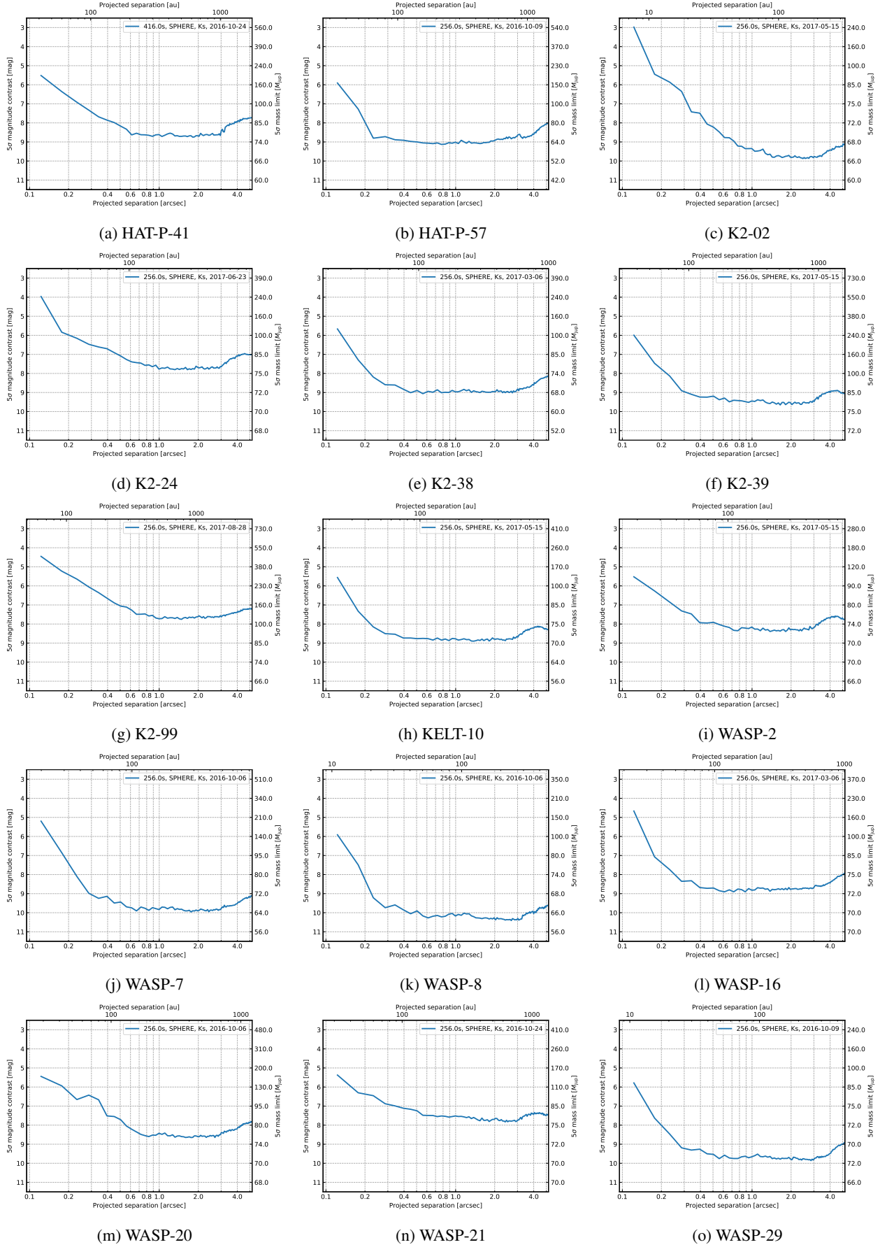
Fig. A.1: Detection limits of individual targets I. We convert projected angular separations in projected physical separations by using the distances presented in Table 1. The mass limits arise from comparison to AMES-Cond, AMES-Dusty, and BT-Settl models as described in Sect. 4.2.
