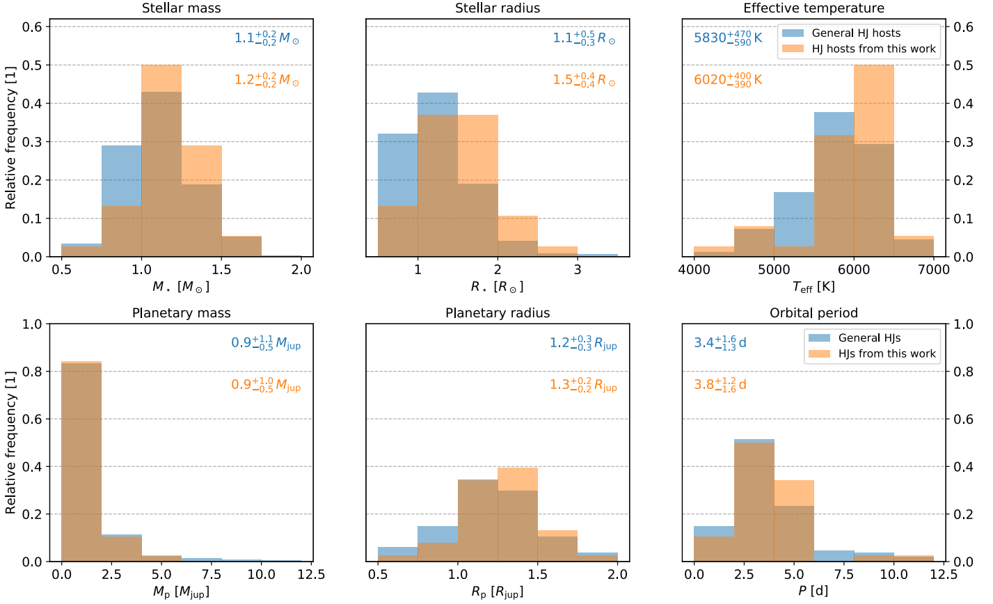
Fig. 11: Histograms of hot Jupiter (HJ) system properties. We compare the targets analysed within the scope of this study (orange bars) to a general sample of hot Jupiter environments (blue bars). In the top panel the relative frequency distributions of stellar masses M_* , radii R_* , and effective temperatures T_{\text{eff}} amongst both samples are presented. The lower panel shows properties of the transiting companions such as planetary masses M_p , planetary radii R_p , and orbital periods P instead. In the upper part of each plot, we present the 68 % confidence intervals around the medians of the corresponding distributions.
