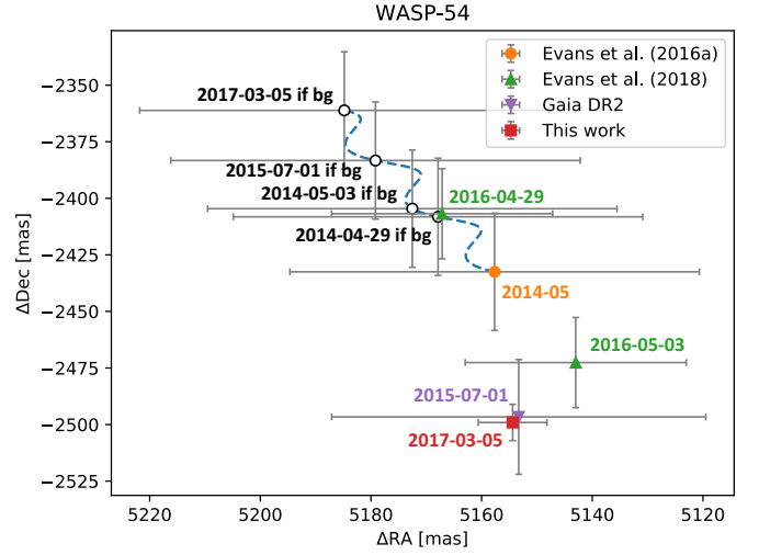
Fig. 5: Proper motion analysis of CC 1 around WASP-54. The first measurement from Evans et al. (2016a) (orange circle) is the average of four individual epochs, collected from May 6 until May 8, 2014. The dashed blue line represents the trajectory of a static background (bg) object.
