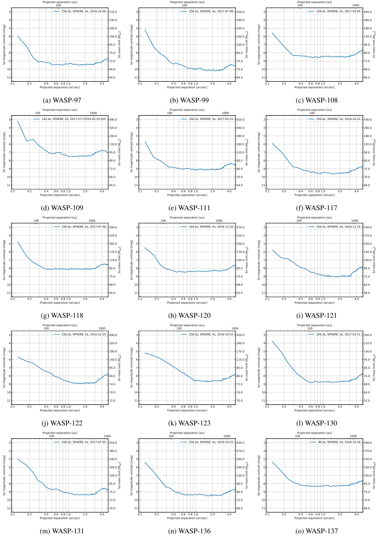
Fig. A.3: Detection limits of individual targets III. We convert projected angular separations in projected physical separations by using the distances presented in Table 1. The mass limits arise from comparison to AMES-Cond, AMES-Dusty, and BT-Settl models as described in Sect. 4.2.
