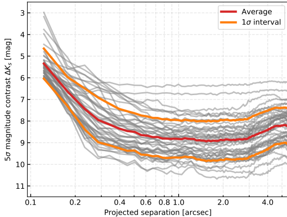
Fig. 10: Detection limits of our SPHERE survey for detection of stellar companions to known exoplanet host stars. The grey lines represent all individual targets and epochs as presented in Table 2 and the red curve and orange curves indicate the average contrast performance and the corresponding 1\sigma interval.
