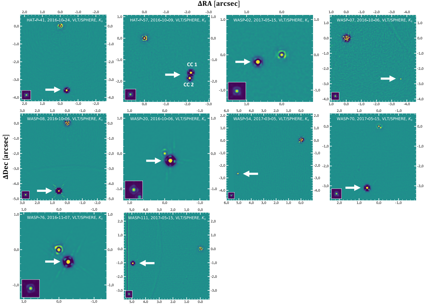
Fig. 2: Previously detected candidate companions around transiting exoplanet host stars from the SPHERE/IRDIS data. An unsharp mask was applied to highlight point sources. The origin of the axes is located at the position of the host star. The images are displayed using a logarithmic scale with arbitrary offsets and stretches to highlight the candidate companions. In all images north points up and east towards the left. The lower left corner of each image shows the reduced non-coronagraphic flux image with the same spatial scale and field orientation.
