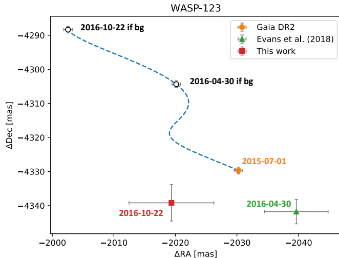
Fig. 9: Proper motion analysis of CC 1 around WASP-123. The dashed blue line represents the trajectory of a static background (bg) object.
