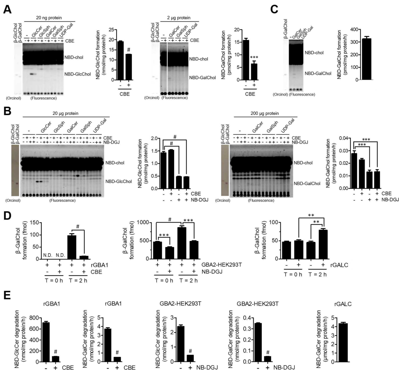
Figure 9. Assessment of in vitro transglycosylation activity of GBA1, GBA2, and GALC in the presence of various glycosyl donors. A–C , in vitro transglycosylation of NBD-GlcChol and NBD-GalChol by GBA1, GBA2, or GALC. rGBA1, homogenates derived from GBA2-overexpressing HEK293T cells or rGALC were incubated for 2 h with NBD-chol and GlcCer (d18:1-C18:1), GlcSph and GalCer (d18:1-C12:0), GalSph, or UDP-Gal as glycosyl donors. The samples were also incubated in the absence or presence of respective specific \beta -glucosidase inhibitors as follows: 0.5 mM CBE (for GBA1) and/or 0.3 mM NB-DGJ (for GBA2). Formation of NBD-GlcChol and NBD-GalChol was detected by HPTLC and fluorescence scanning. NBD-GlcChol and NBD-GalChol were identified by co-chromatography using authentic standards of \beta -GlcChol and \beta -GalChol, respectively. The authentic standards were visualized by spraying the HPTLC plates with orcinol reagent. Bar graphs show the concentrations of NBD-GlcChol formed in the presence of NBD-chol and GlcCer (d18:1-C18:1) and the concentrations of NBD-GalChol formed in the presence of NBD-chol and GalCer (d18:1-C12:0). Differences were analyzed by unpaired t tests; ***, p < 0.001 ; #, p < 0.0001 . A , HPTLC analysis showing the quantification of NBD-GlcChol ( left image ) and NBD-GalChol ( right image ) formed in reactions comprising either 20 ng or 2 \mu g of rGBA1 protein as the enzyme source and the indicated glycosyl donors. Data presented as means \pm S.E.; n = 4 . B , HPTLC analysis showing the quantification of NBD-GlcChol ( left image ) and NBD-GalChol ( right image ) formed in reactions comprising either 20 or 200 \mu g of protein in homogenates derived from GBA2-overexpressing HEK293T cells as the enzyme source and the indicated glycosyl donors. Data are presented as means \pm S.E.; n = 4–6 . C , HPTLC analysis showing the quantification of NBD-GalChol formed in reactions comprising rGALC as the enzyme source and the indicated glycosyl donors. Data presented as means \pm S.E.; n = 4 . D , in vitro transgalactosylation of \beta -GalChol by GBA1, GBA2, and GALC. rGBA1, homogenates from GBA2-overexpressing HEK293T cells, or rGALC were incubated for 0 or 2 h with cholesterol in the presence of GalCer (d18:1-C12:0) as glycosyl donor and in the absence or presence of the respective specific \beta -glucosidase inhibitor: 0.5 mM CBE (for GBA1) or 0.3 mM NB-DGJ (for GBA2). Formation of \beta -GalChol was detected by HILIC-ESI-MS/MS. Differences ( n = 4–5 , means \pm S.E.) were analyzed by unpaired t tests. **, p < 0.01 ; ***, p < 0.001 ; #, p < 0.0001 ; N.D. , not detected (below the detection threshold). E , in vitro GlcCer and GalCer hydrolysis activities of GBA1, GBA2, and GALC. rGBA1, homogenates from GBA2-overexpressing HEK293T cells, or rGALC was incubated for 30 min with C_6 -NBD-GlcCer or C_6 -NBD-GalCer and in the absence or presence of the respective specific \beta -glucosidase inhibitor: 0.5 mM CBE (for GBA1) or 0.3 mM NB-DGJ (for GBA2). HPTLC and fluorescence scanning were used to detect C_6 -NBD-ceramide formation. Data presented as means \pm S.E.; n = 4–5 . Differences were analyzed by unpaired t tests; #, p < 0.0001 .
