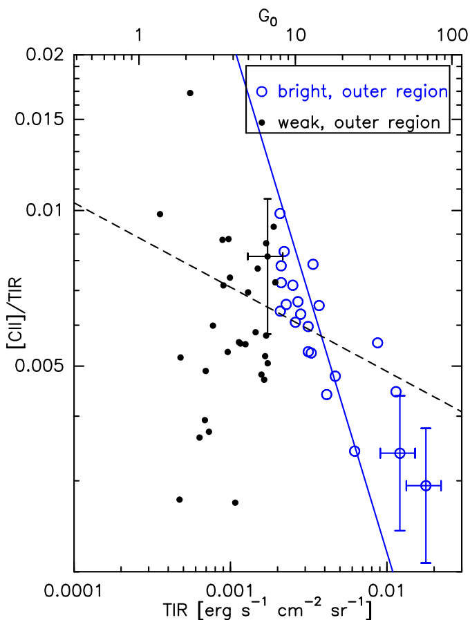
Fig. 9. [C\ II]/TIR intensity ratio versus TIR for the northern H\ II region BCLMP 691 in M 33. The blue drawn line shows the result of an unweighted linear least-squares fit to the TIR-bright data of BCLMP 691 varying only the y-intercept, while keeping the slope fixed at -1 . The black dashed line shows the result of an unweighted linear least-squares fit to all M 33 data (cf. Fig. 5). A few typical 1\sigma errorbars are shown.
