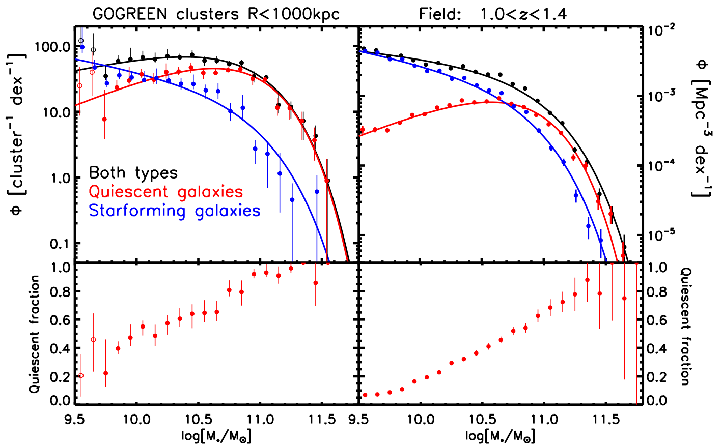
Fig. 4. Top left panel: SMF of cluster galaxies within R \leq 1000 kpc from the cluster centres. Black points: Total galaxy population. Blue and red data points: The population of star-forming and quiescent galaxies, respectively. Small horizontal offsets have been applied compared to the black points for better visibility. The open circles mark points below the 80% mass completeness limit, and, even though we perform an incompleteness correction, these are, conservatively, not used in the fitting. Top right panel: SMF of co-eval field galaxies from the COSMOS/UltraVISTA survey ( 1.0 < z < 1.4 ). The best-fitting Schechter functions are included in both top panels. Lower panels: Relative fraction of quiescent galaxies as a function of stellar mass, in the different environments.
