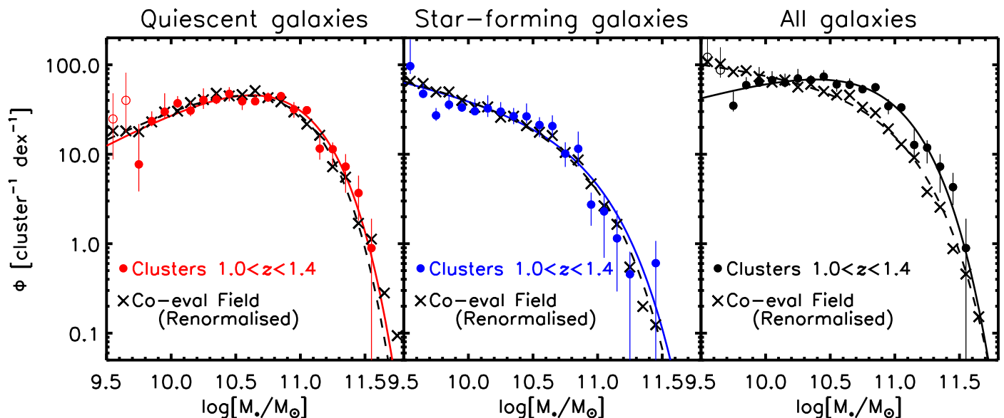
Fig. 6. Left: The SMF function of quiescent galaxies in the cluster environment ( R < 1000 kpc), compared to the field. The cluster data points are identical to those shown in Fig. 4, while the field is normalised so that it integrates to the same number of quiescent galaxies down to M_* \geq 10^{9.5} M_\odot . Middle: Same but for star-forming galaxies. The best-fitting Schechter functions are over-plotted. The resemblance in the shapes of the separate (quiescent versus star-forming galaxies) SMFs is evident. Right: Same comparison but for all galaxies, where there clearly is a different SMF between cluster and field.
