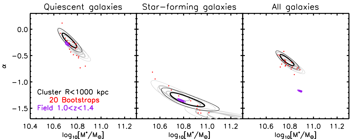
Fig. 5. Comparison of the best-fitting Schechter parameters between cluster and field, when the galaxy population is divided between different galaxy types. Black contours : 1- and 2- \sigma uncertainties corresponding to the main analysis. Grey : Robustness tests based on different initial photometric selection of cluster members. Red dots : Results based on cluster bootstrap samples, where clusters are drawn with replacement. Purple contours : 1- and 2- \sigma uncertainties for the co-eval reference field.
