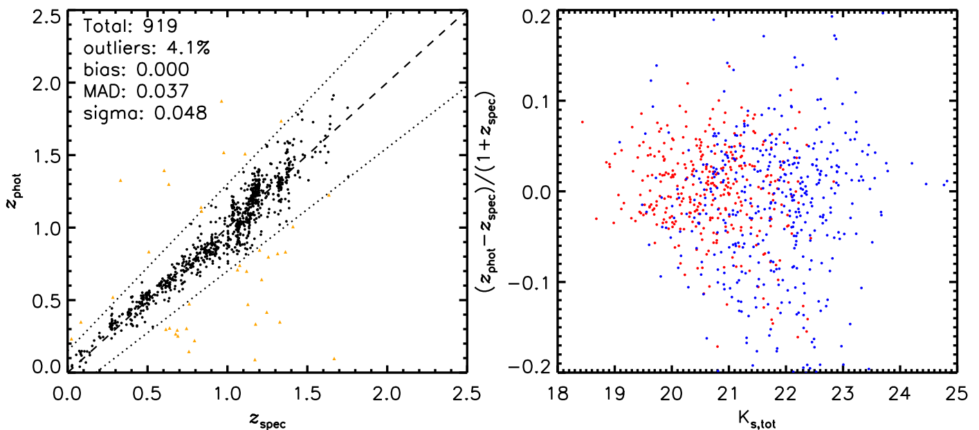
Fig. 1. Left: Photometric versus spectroscopic redshifts for all galaxies in the 11 cluster fields. Outliers, defined as objects for which |\Delta z| > 0.15 , are marked in orange. The outlier fraction is 4.1%, the scatter of the remaining objects is \sigma_z = 0.048 . Right: \Delta z as a function of K_s -band magnitude, for sources with 1.0 < z_{\text{spec}} < 1.5 . Quiescent and star-forming galaxies (separated according to the criteria given in Sect. 3.3) are marked in red and blue, respectively.
