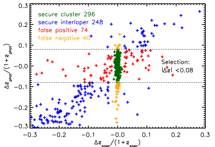
Fig. 3. The same information as in Fig. 1, but here the x-axis shows the difference in z_{\text{spec}} with respect to the cluster redshift. This way we can identify spectroscopic cluster members (orange and green), as well as photometric cluster galaxies (red and green). Our fiducial measurement approach subtracts fore- and background interloper galaxies based on these relative numbers, after splitting the sample by galaxy type, and selecting similar sources in terms of stellar mass and projected radial distance from the cluster centers (cf. A.2).
