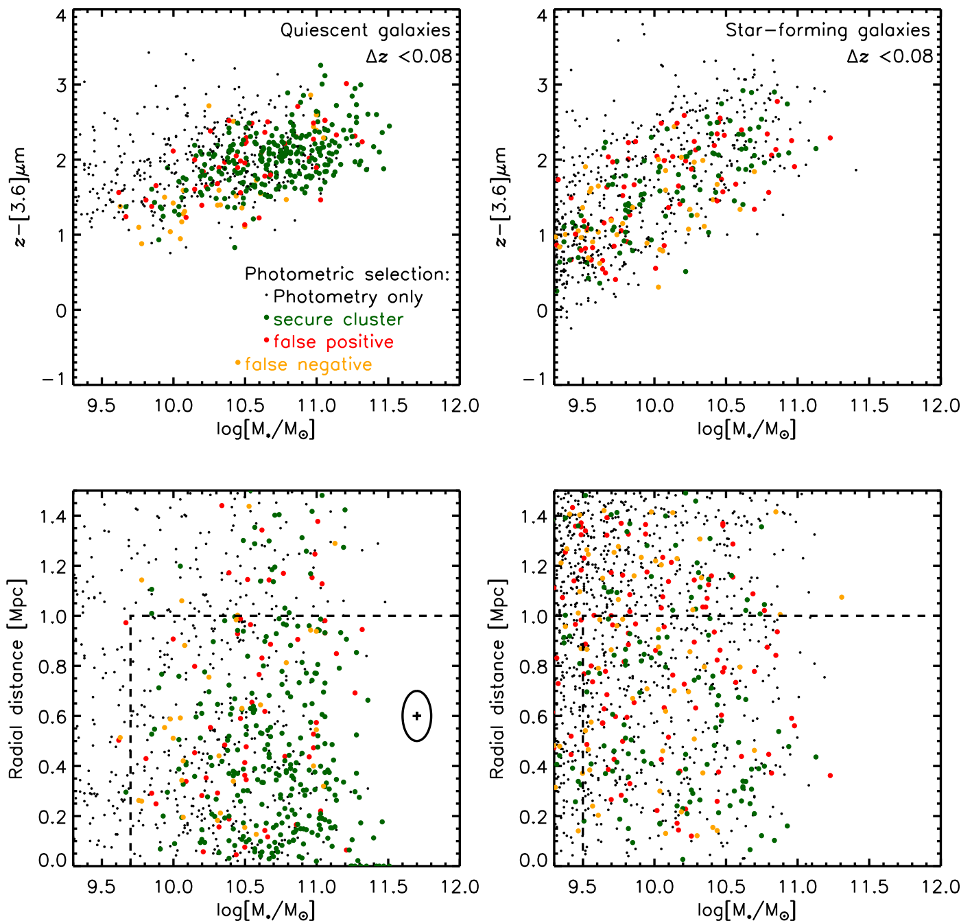
Fig. A.2. Top panels: Colour- stellar mass diagram that compares the spectroscopic targets (coloured points) with photometrically selected cluster galaxy candidates (black+green+red). Our method of subtracting fore- and background interlopers relies on the spectroscopic subset being a representative subset. Left panel: Quiescent galaxies, for which this criterion is not fully met at low masses. Right panel: Star-forming galaxies, for which this assumption is valid. Lower panels: Spectroscopic targets shown as a function of cluster-centric distance and stellar mass. The ellipse shows the relative weight we give to either parameter when defining the five closest sources in this plane (which are used to estimate membership for the black points). Dashed region defines the population studied in this work.
