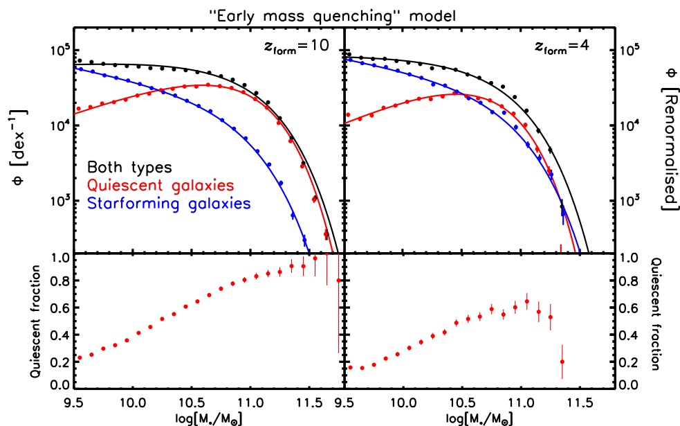
Fig. 9. Top panels: The result of a galaxy evolution models following the formalism for mass quenching, as described in Peng et al. (2010). These assume a formation redshift of z_{\text{form}} = 10 (left panel) and z_{\text{form}} = 4 (right panel), and the panels compare the results at z = 1.2 . For easy comparison, the right panel was renormalised by a factor 5.6 so that both panels have the same number of galaxies in the plotted mass range. Lower panels: Relative fraction of quiescent galaxies for the model runs with the two different formation redshifts. In this model we observe a qualitatively similar SMF of quiescent galaxies in both panels, as well as for the star-forming galaxies. Moreover, the mass-dependent QFE of the z_{\text{form}} = 10 population compared to the z_{\text{form}} = 4 population is similar to what we observe (cf. Fig. 7). Details on the model are given in Sect. 5.2 and in Peng et al. (2010).
