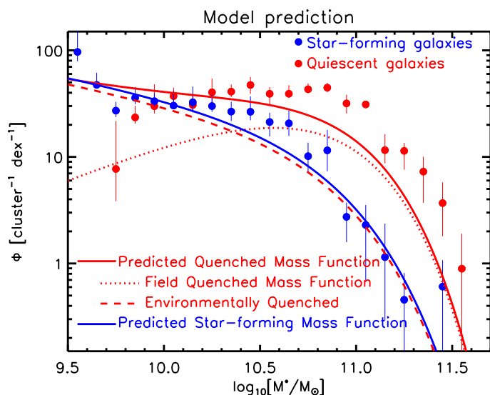
Fig. 8. A comparison between the data and predictions from the model described in Sect. 5.1. The main model assumption is that the quenched fraction excess is independent of stellar mass, and fixed to the best-fit value of QFE = 0.47 \pm 0.03 . This corresponds to the pure environmental quenching scenario from Peng et al. (2010), but is contrary to the mass dependence we observe, cf. Fig. 7. While the star-forming SMF is well reproduced by this model, there is a clear mis-match between the predicted (red solid line) and observed (red points) SMF of quiescent (cluster) galaxies.
