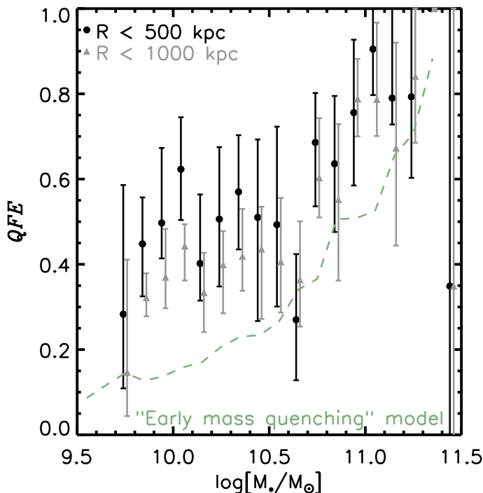
Fig. 7. Quenched Fraction Excess ( QFE ) for cluster galaxies as a function of stellar mass. Black: Considering cluster galaxies at R < 500 kpc. Grey: Considering cluster galaxies at R < 1000 kpc. Green dashed: Galaxy evolution model as described in Sect. 5.2, where the field and cluster galaxies have started forming at different redshifts.
