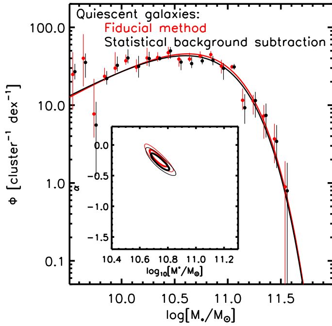
Fig. B.1. Red : Our fiducial analysis makes best use of the spectroscopic coverage of GOGREEN. It reduces the effect of cosmic variance since it does not rely on the statistical subtraction of interlopers from a reference field. However, for this approach we have to assume that the spectroscopic subset is representative of the full galaxy population. Black : An alternative approach is to subtract the fore- and background interlopers statistically by making use of the external COSMOS/UltraVISTA survey. The latter approach does not make use of the spectroscopy at all, yet presents results that are fully consistent with those obtained with the fiducial method. Small horizontal offsets have been applied, to the data points only, for better visibility.
