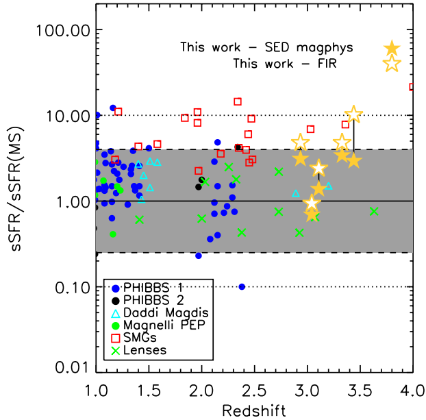
Figure 1. sSFR, normalized to the one estimated for the main sequence (sSFR(MS)) as a function of redshift, for different samples of normal “main sequence” galaxies with at least one CO line detected in their spectra. Blue points and black points show, respectively, galaxies from the PHIBBS 1 survey (Tacconi et al. 2010, 2013), and PHIBBS 2 survey (Combes et al. 2016); red squares indicate SMGs from Greve et al. (2005), Tacconi et al. (2006), Tacconi et al. (2008), Bothwell et al. (2013); cyan triangles indicate star-forming BzK objects from Daddi et al. (2010) and Magdis et al. (2012); filled green circles are galaxies from Magnelli et al. (2012); green crosses indicate lensed galaxies from Saintonge et al. (2013) and Dessauges-Zavadsky et al. (2017). Yellow stars show the five objects presented in this work: filled stars indicate the SFR that is obtained by the MAGPHYS tool; empty stars indicate the star formation rates that are obtained converting the L_{FIR} using the classical Kennicutt relation. The horizontal continuous line marks the location of the MS, the dashed (dotted) lines indicate the locii 4x (10x) times above or below the MS. The grey area emphasizes the location of the main sequence, according to the classical definition by Rodighiero et al. (2011; 2014), and Elbaz et al. (2018).
