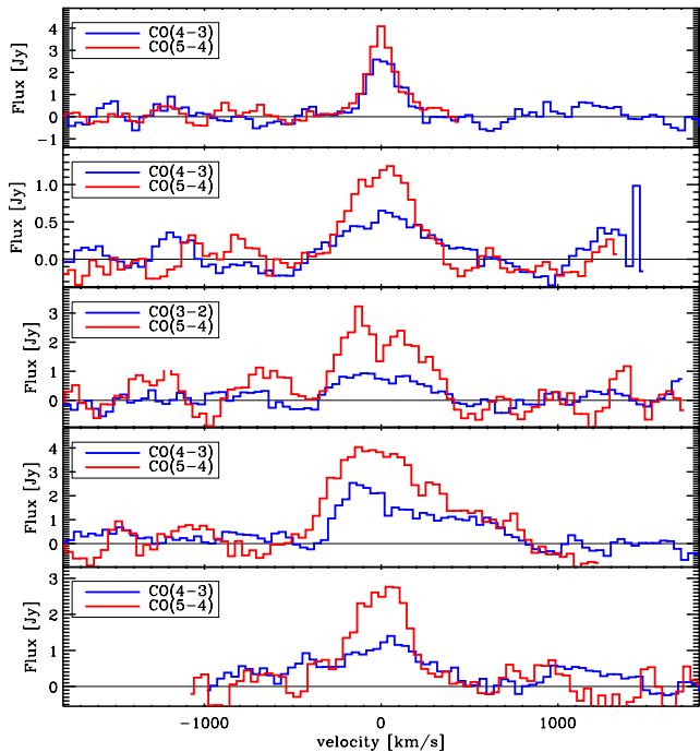
Figure 3. Mm/sub-mm spectra of the five sample galaxies in band 4 (red) and band 3 (blue), highlighting, respectively, the CO(5-4) emission and the CO(4-3) (for objects 1, 2, 4 and 5) or CO(3-2) (for object 3). The spectra, extracted in channels of 40 km/s, are expressed in Jy as a function of the velocity offset from the redshift centered on the CO(5-4) line, and are extracted from the region over which we integrate the moment 0 maps to obtain the total line fluxes. In each panel, we report the FWHM of the CO(5-4) line emission.
