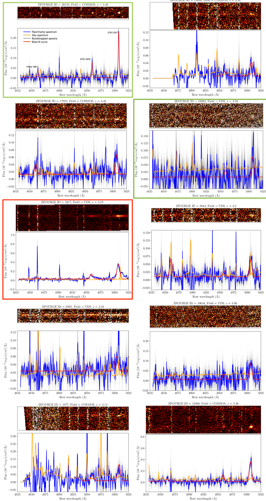
Figure 10. Same as Figure 1 but for all the 10 galaxies with \log(M_*/M_\odot) > 10.2 . Spectra of two galaxies with unphysical dynamical masses are highlighted with green box. The spectrum highlighted with a red box corresponds to a possible AGN contaminant.
