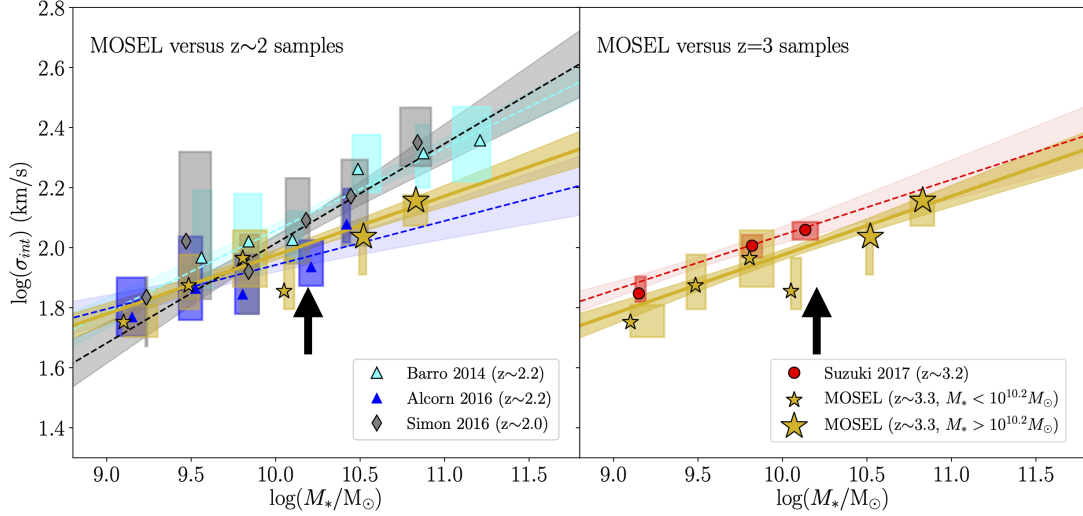
Figure 5. The Integrated velocity dispersion ( \log(\sigma_{\text{int}}) ) for the MOSEL galaxies (gold stars) binned into stellar mass in comparison with the sample at z \sim 2 (left) and z > 3 (right). The color scheme is the same as in Figure 4. The symbols and the shaded rectangles correspond to the median and the 25 th to 75 th percentile in \log(\sigma_{\text{int}}) and stellar mass after bootstrapping respectively. The dashed lines represent the best-fit linear relation between M_* and \log(\sigma_{\text{int}}) for the respective sample. Massive galaxies with \log(M_*/M_\odot) > 10.2 (pointed by the black arrow) from our MOSEL survey have lower \log(\sigma_{\text{int}}) compared to galaxies of similar stellar masses at z \sim 2 .
