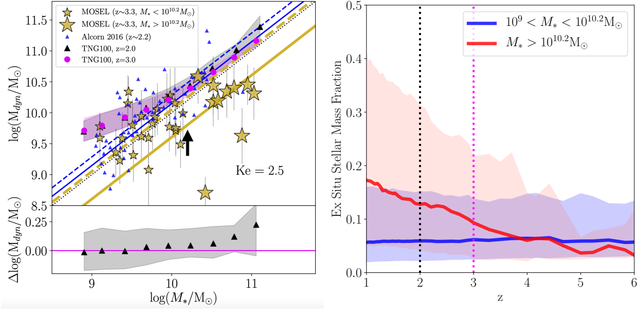
Figure 9. Left panel: Comparison between the dynamical to stellar mass relation in observations and simulations. The color scheme and symbols are the same as Figure 8. The black dotted line is the one-to-one line. The colored dashed and solid lines represent the average offset in the dynamical mass of low and high mass (split at \log(M_{*}/M_{\odot}) = 10.2 , pointed by the black arrow) galaxies in the respective samples from the one-to-one line. The bottom panel shows the change in the dynamical mass at a fixed stellar mass between z = 2 - 3 , showing the \sim 0.1 dex increase in the dynamical mass at z = 2 for massive galaxies. Right panel: The ex situ stellar mass fraction (accreted) with respect to redshift for low mass ( 9.0 < \log(M_{*}/M_{\odot}) < 10.2 , blue) and high mass sample ( \log(M_{*}/M_{\odot}) > 10.2 , red) in the TNG100 simulation. The solid line and shaded region represent the median and, 16 th , and 84 th percentiles, respectively. The pink and black dotted lines mark the redshift snapshots of z = 3 and z = 2 respectively. The ex situ stellar mass fraction increases sharply below z < 3.5 for massive galaxies.
