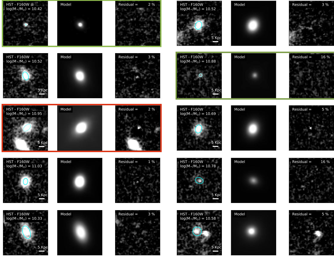
Figure 11. Same as Figure 2 but for all the 10 galaxies with \log(M_*/M_\odot) > 10.2 . The HST-F160W image and GALFIT models highlighted with green and red boxes correspond to galaxies with unphysical dynamical masses and possible AGN contaminant, respectively.
