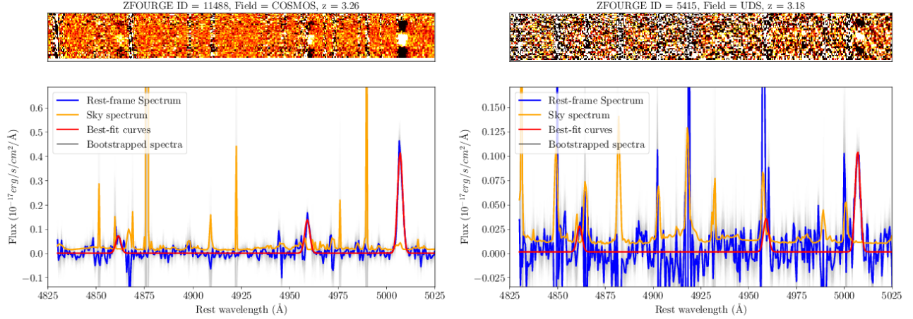
Figure 1. Sample spectra for two MOSEL galaxies from MOSFIRE observations. The blue curves are the observed 1D spectra in the rest frame, orange is corresponding noise spectra, and the gray shaded region is the bootstrapped iterations. The red curves correspond to the best-fit curves to the [O III] \lambda\lambda 5007, 4959 and H \beta\lambda 4861 emission lines. The image in top panel shows the corresponding 2D spectrum for each galaxy. We provide MOSFIRE spectra of all massive MOSEL galaxies in Appendix 10.
