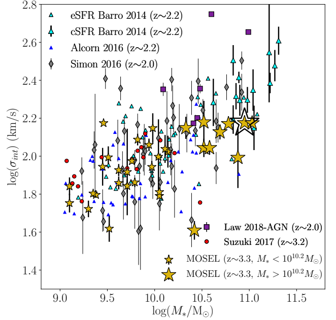
Figure 4. Left : Distributions of the integrated velocity dispersion ( \log(\sigma_{int}) ) versus stellar mass for the MOSEL galaxies (gold stars). The small and large gold stars correspond to the two sub-groups identified using the k-Means clustering algorithm separated at a stellar mass of M_* = 10^{10.2} M_\odot . The big open star corresponds to a galaxy with broad emission features indicative of an AGN. We compare the MOSEL sample with SFGs at z \sim 2 from Barro et al. (2014), Alcorn et al. (2016), and Simons et al. (2016). Additionally, we compare with SFGs at z \sim 3 from Suzuki et al. (2017) and AGNs at z \sim 2 from Law et al. (2018).
