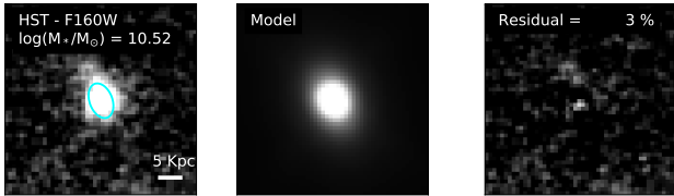
Figure 2. HST-F160W image (left) of a sample galaxy from the MOSEL survey. The middle and the right panels show the best-fit spatial profiles and residuals, respectively from GALFIT. The cyan ellipse in the left panel indicates the best-fit ellipse along the semimajor axis with a radius equal to the twice the effective radius. The legend in the right panel indicates the percentage residuals summed in quadrature within twice the effective radius. For velocity dispersion and dynamical mass analysis, we select galaxies with the total percentage residuals < 20\% . We provide GALFIT models for all massive MOSEL galaxies in Appendix 11.
