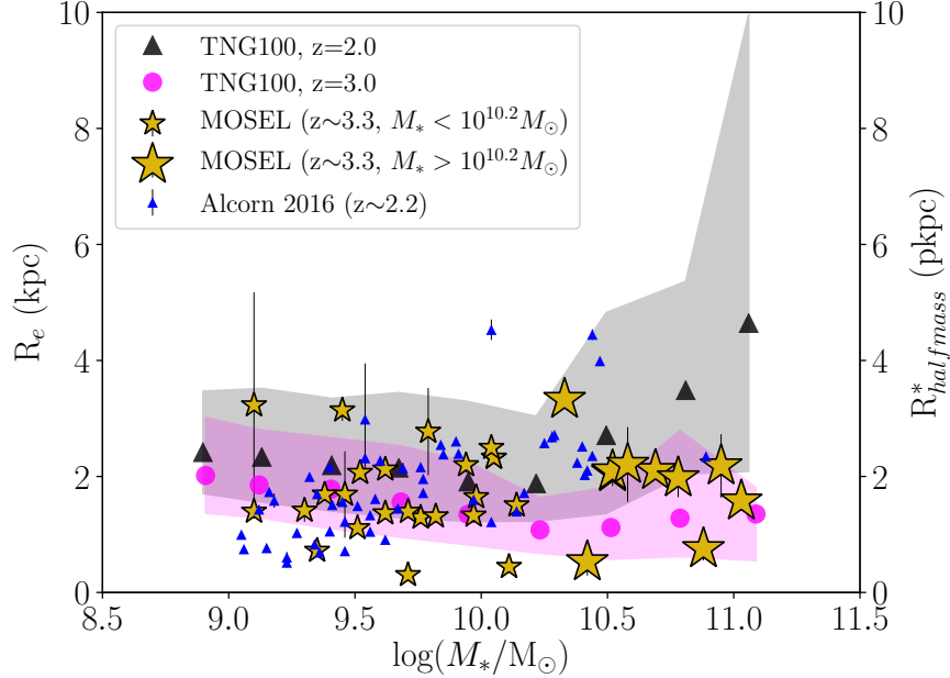
Figure 8. Comparison between HST-F160W effective radii ( R_e ) from observations and R_{halfmass}^* from the TNG100 simulation as a function of the stellar mass. The large and small golden stars correspond to the MOSEL galaxies with \log(M_*/M_\odot) > 10.2 and \log(M_*/M_\odot) < 10.2 respectively. The pink circles and shaded region represent the 50 th , 16 th and 84 th percentile in the R_{halfmass}^* from TNG100 at z = 3.0 . Similarly, the black triangles and gray shaded region represent the R_{halfmass}^* at z = 2.0 in TNG100.
