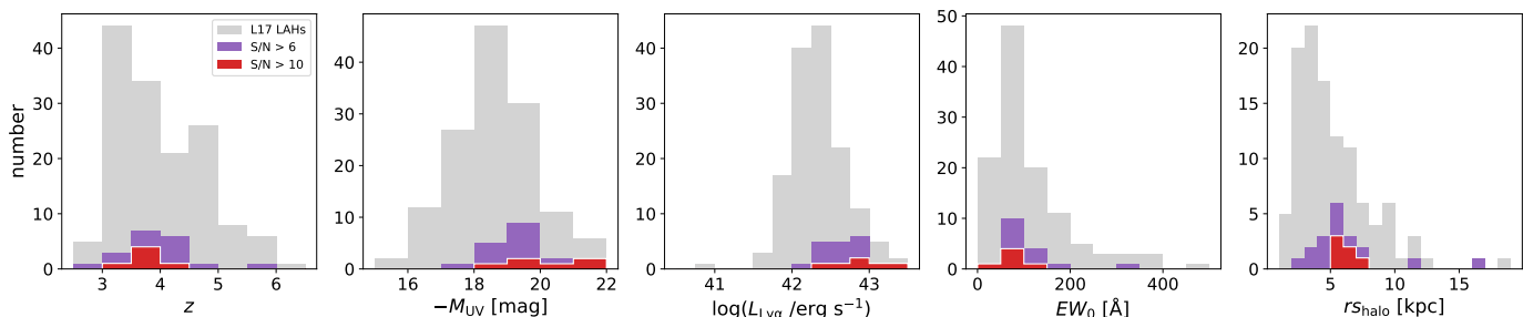
Fig. 1: From left to right: Redshift, absolute UV magnitude, Ly \alpha luminosity, Ly \alpha rest-frame equivalent width, and Ly \alpha halo scale length distributions of the parent sample (grey), the S/N > 6 (purple) and the S/N > 10 (red) samples.
