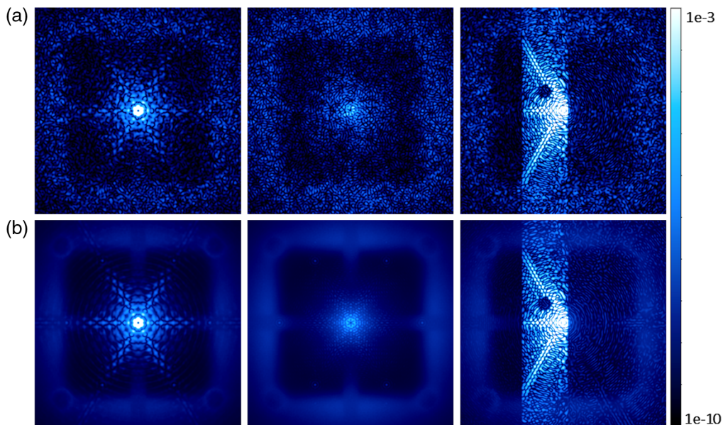
Fig. 9 (a) Representative instantaneous PSFs at the L-band, using a single SCAO residual phase screen obtained in the cases of CVC (left), RAVC (center), and APP (right). (b) Same for long-exposure PSFs, averaged over the 1-h SCAO sequence. All images have been cropped to a field of view of 100\lambda/D , i.e., 2.1'' at the L-band. All PSFs have been normalized by the maximum intensity in the noncoronagraphic PSF of the corresponding HCI mode. The dark spot in the APP PSF was purposely created on the optical axis to enable high-SNR measurements of the so-called leakage term (not included here), a scaled-down version of the stellar PSF due to imperfection in the phase shift induced by liquid crystals, which can be used to monitor the photometry and astrometry of the central star without saturating the detector.
