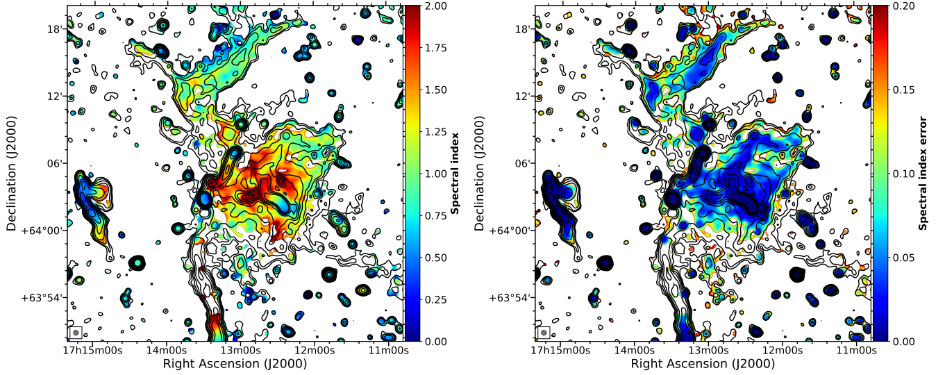
Figure 5. Spectral index map between 144 MHz and 1.2 GHz of the central radio emission in A2255 at a resolution of 28'' \times 28'' ( left ) with the corresponding (statistical) error map ( right ). LOFAR contours at the same resolution starting from 360 \mu\text{Jy beam}^{-1} and spaced by a factor of 2 are shown. Pixels with values below 3\sigma were not considered in the computation of the spectral index.
