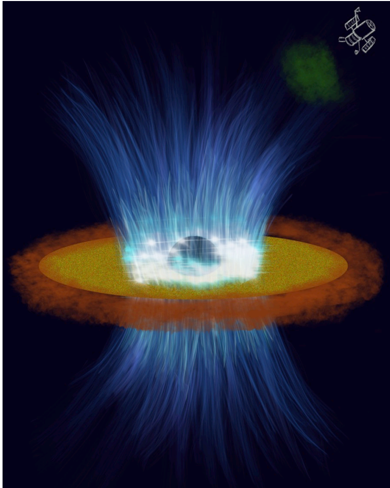
Figure 5. Cartoon of the disk wind in NGC 5548 (not to scale). The disk wind (blue) surrounds the central black hole and extends to the line of sight to HST in the upper right corner. The BLR is shown as the orange cloud around the disk. The green cloud at the upper right shows the absorbing cloud discussed in D19a. The bright region in the lower part of the wind indicates that the wind is a major contributor to the very broad components of the observed emission lines
