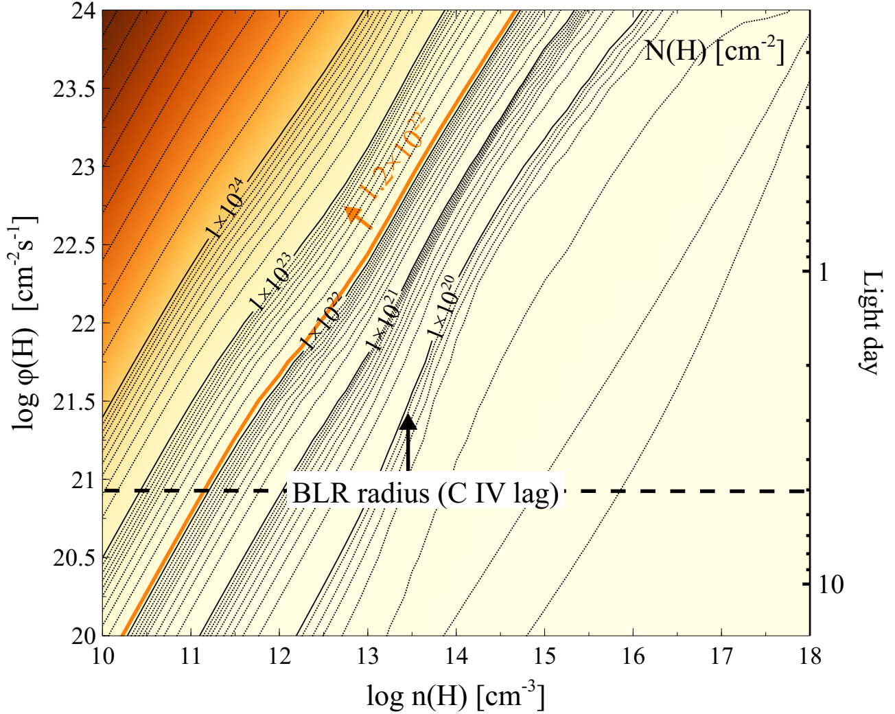
Figure 1. The contours show total hydrogen column density of the equatorial obscurer as a function of the flux of ionizing photons and the hydrogen density. The orange line indicates the LOS obscurers column density (D19a) and the dashed black line shows the location of the BLR based on the observed C IV lag.
