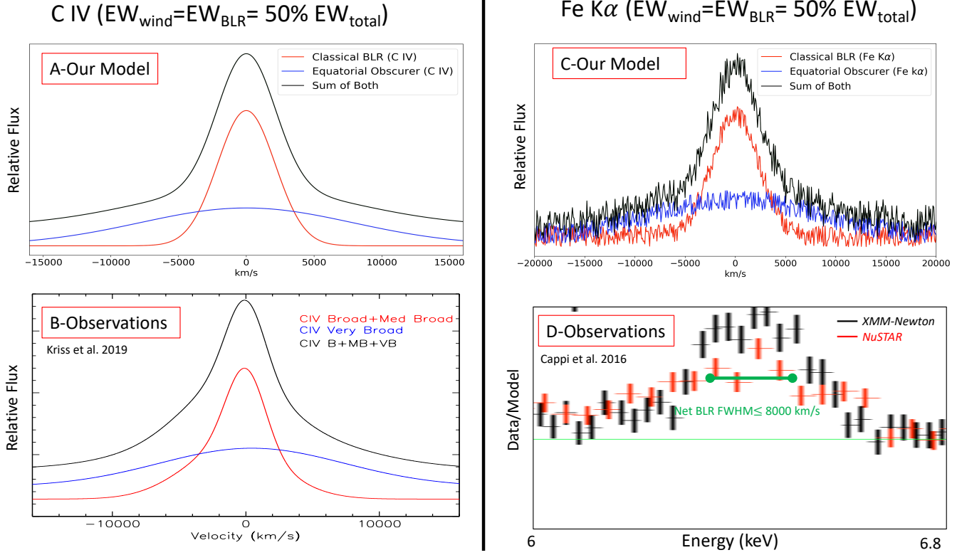
Figure 4. This Figure compares our model with the observations from HST , XMM-Newton , and NuSTAR . Panels A & B show the case for C IV, for which the obscurer produces a very broad component (panel A, blue) with an EW of half of that produced by the BLR (panel A, red). Panels C & D show the case for Fe K \alpha , for which the obscurer produces a very broad component (panel C, blue) with an EW equal to that produced by the BLR (panel C, red). It is plausible that a broad base similar to C IV is present, although the S/N is not high enough to say for sure. In both cases our predictions are very similar to the observations, suggesting that the disk wind could be responsible for the observed very broad emission line components.
