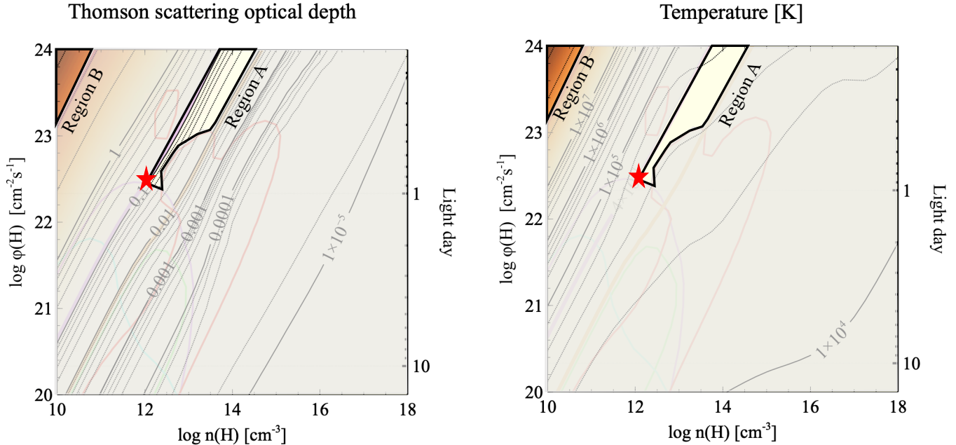
Figure 3. The left panel maps the Thomson scattering optical depth and the right panel maps the temperature of the obscurer. A and B are two regions with allowed properties of the equatorial obscurer. The red star indicates our preferred model, which is the most consistent with all observational constraints
