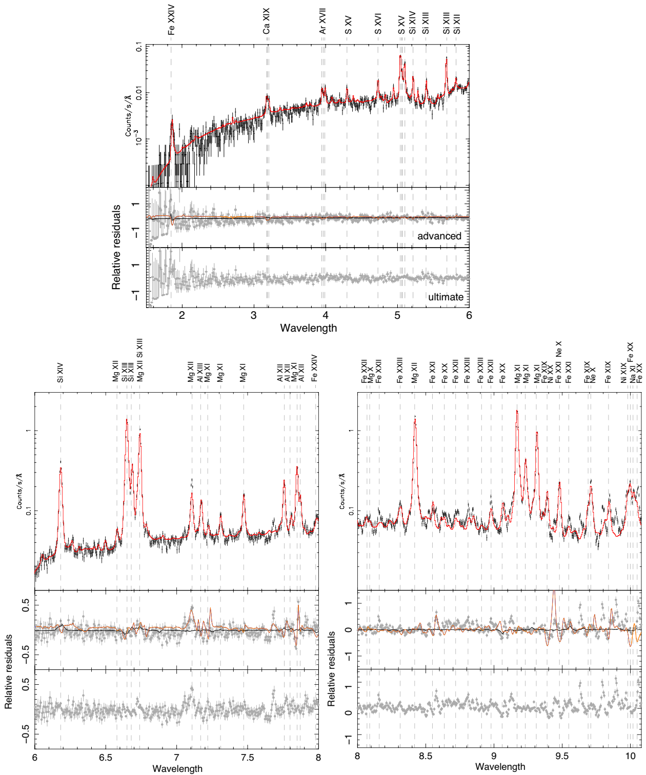
Fig. B.1. Chandra grating spectrum of Capella in 1.5 - 10.08 \text{ \AA} fit with different models. Upper panels in each subfigure show fit with the advanced SPEX-ADAS model with EBIT calibration (red). Middle panels show the fit residual with the advanced models (grey points), as well as the ratio between the SPEX-FAC fit and the SPEX-ADAS fit in black, and the APEC-to-SPEX-ADAS ratio in orange. Lower panels show the fit residual with the ultimate model.
